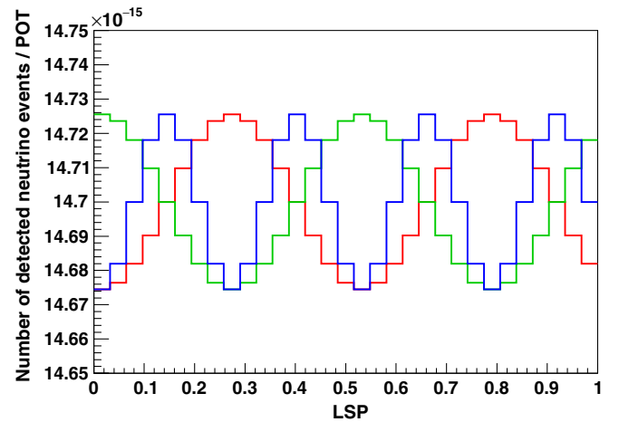
FIG. 4. Distribution of the \nu_\mu event rate as a function of LSP for three different assumed signal configurations: (\mathcal{C}_{\mu e}, \mathcal{A}_c)_{\mu e}, (\mathcal{A}_s)_{\mu e}, (\mathcal{B}_c)_{\mu e}, (\mathcal{B}_s)_{\mu e} = (0, 5 \times 10^{-20}, 0, 0, 0) GeV (red), (0, 0, 5 \times 10^{-20}, 0, 0) GeV (green), and (0, 0, 0, 5 \times 10^{-20}, 0) GeV (blue). The coefficients corresponding to \nu_\mu \rightarrow \nu_\tau oscillation (\mathcal{C}_{\mu\tau}, \mathcal{A}_c)_{\mu\tau}, (\mathcal{A}_s)_{\mu\tau}, (\mathcal{B}_c)_{\mu\tau}, (\mathcal{B}_s)_{\mu\tau} have been set to zero.
