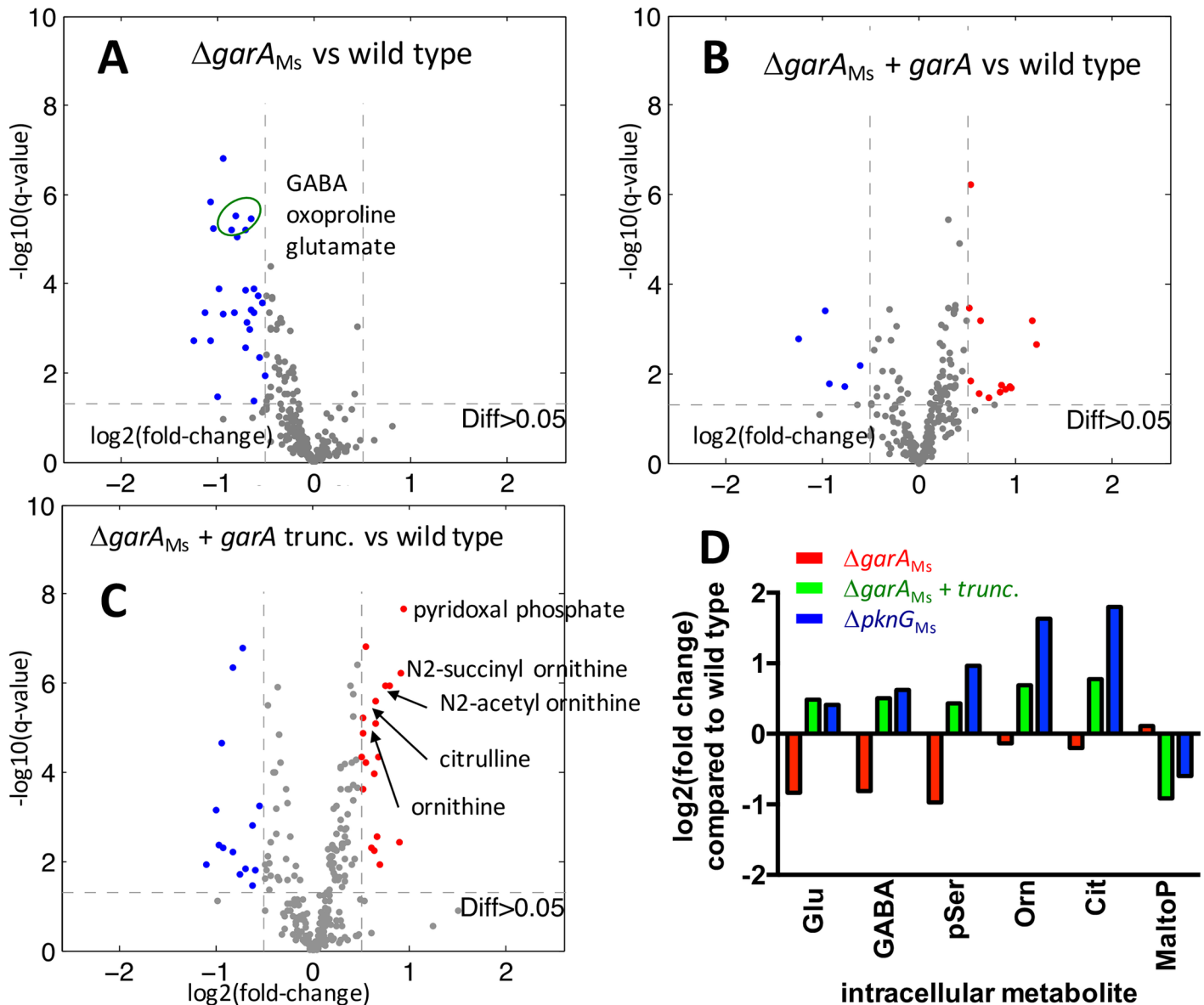
Fig 7. Deletion of garA or disruption of GarA phosphorylation caused changes in intracellular glutamate and other changes in the metabolome of M. smegmatis . Intracellular metabolites from wild type M. smegmatis and mutants were analysed by mass spectrometry using an untargeted metabolomics approach. M. smegmatis lacking garA has lower intracellular glutamate and metabolites related to glutamate than the parental strain (A) but plasmid encoded GarA reversed this change (B). M. smegmatis expressing truncated GarA that lacks phosphorylation sites had higher intracellular ornithine than wild type (C). Intracellular glutamate concentrations for the mutant strains are compared to wild type in panel (D), together with those metabolites that were significantly changed in >1 mutant strain but not in complemented strains. pSer is O-phosphoserine, Orn is ornithine, Cit is citrulline, MaltoP is maltopentaose. (A-C) Each point on the scatter plots represents a single metabolite. Metabolites with the greatest fold-change and statistical significance are highlighted ( \log_2(\text{fold change}) > 0.5 and q\text{-value} < 0.05 ), thresholds marked as dashed lines on graphs); metabolites at lower concentration are blue and those at higher concentration are red. These data were taken from cells growing in Middlebrook 7H9 in early exponential phase and represent the mean from at least 3 independent experiments.
