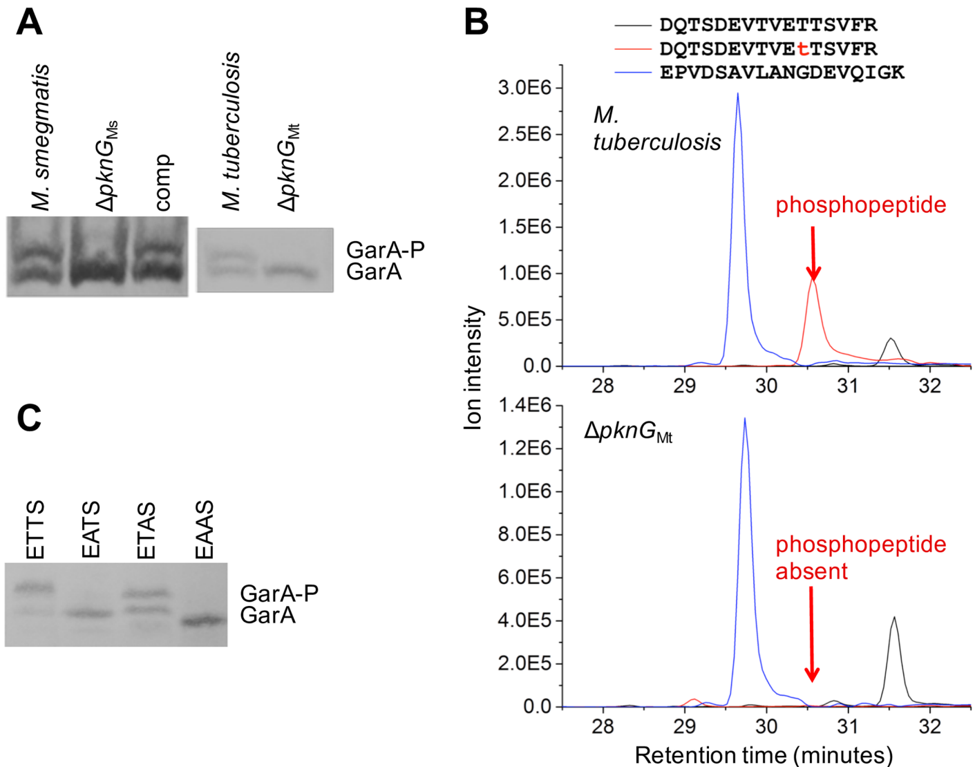
Fig 4. Investigation of GarA phosphorylation in M. smegmatis and M. tuberculosis . (A) Addition of Phos-tag reagent to SDS-PAGE allowed separation of phosphorylated GarA (GarA-P) from GarA. Cell extracts were prepared from M. smegmatis and M. tuberculosis wild type and pknG deletion strains and complemented strains. (B) The same cell extracts of M. tuberculosis wild type and pknG deletion strain were analysed by LC-MS/MS to detect the tryptic peptide of GarA carrying the ETTS phosphorylation motif. The abundance of the peptide with no phosphorylation is shown in black and the T21-phosphorylated peptide is shown in red. A peptide from another part of the protein was also measured as a control (blue). (C) A reporter strain of \Delta garA_{Ms} carrying plasmids encoding hexahistidine-tagged garA , or variants of garA , confirmed that most phosphorylation occurred at the first threonine in the ETTS motif. GarA from cell lysates was visualised by Western blotting. Images shown are representative of three or more independent replicates.
