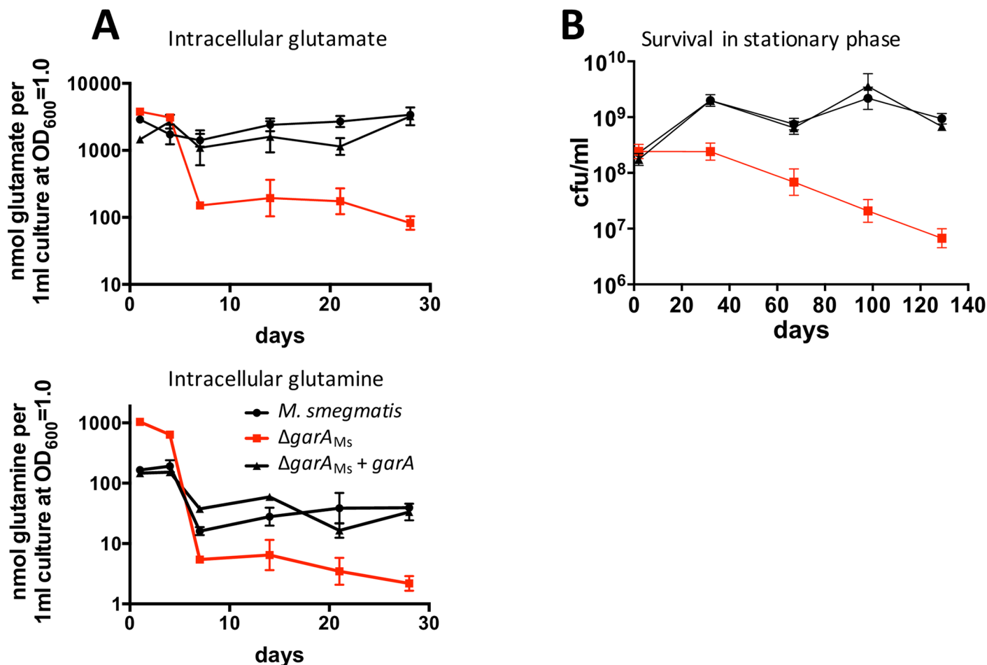
Fig 6. GarA was required during stationary phase for the maintenance of intracellular glutamate and for survival. (A) M. smegmatis lacking garA failed to maintain intracellular glutamate and glutamine pools during extended stationary phase in 7H9 medium. Intracellular glutamate and glutamine were measured for wild type M. smegmatis (black circles), \Delta garA_{Ms} (red squares), and complemented \Delta garA_{Ms} (black triangles). Inset graphs show intracellular metabolites for the same experiment at day 28 (B) M. smegmatis lacking garA gradually lost viability during prolonged stationary phase. Cells were cultured in 7H9 medium over a time period of five months. Aliquots were withdrawn at regular intervals and surviving cells were plated on 7H10 to calculate CFU ml -1 . All experiments were repeated at least 3 times and data show the mean with standard deviation.
