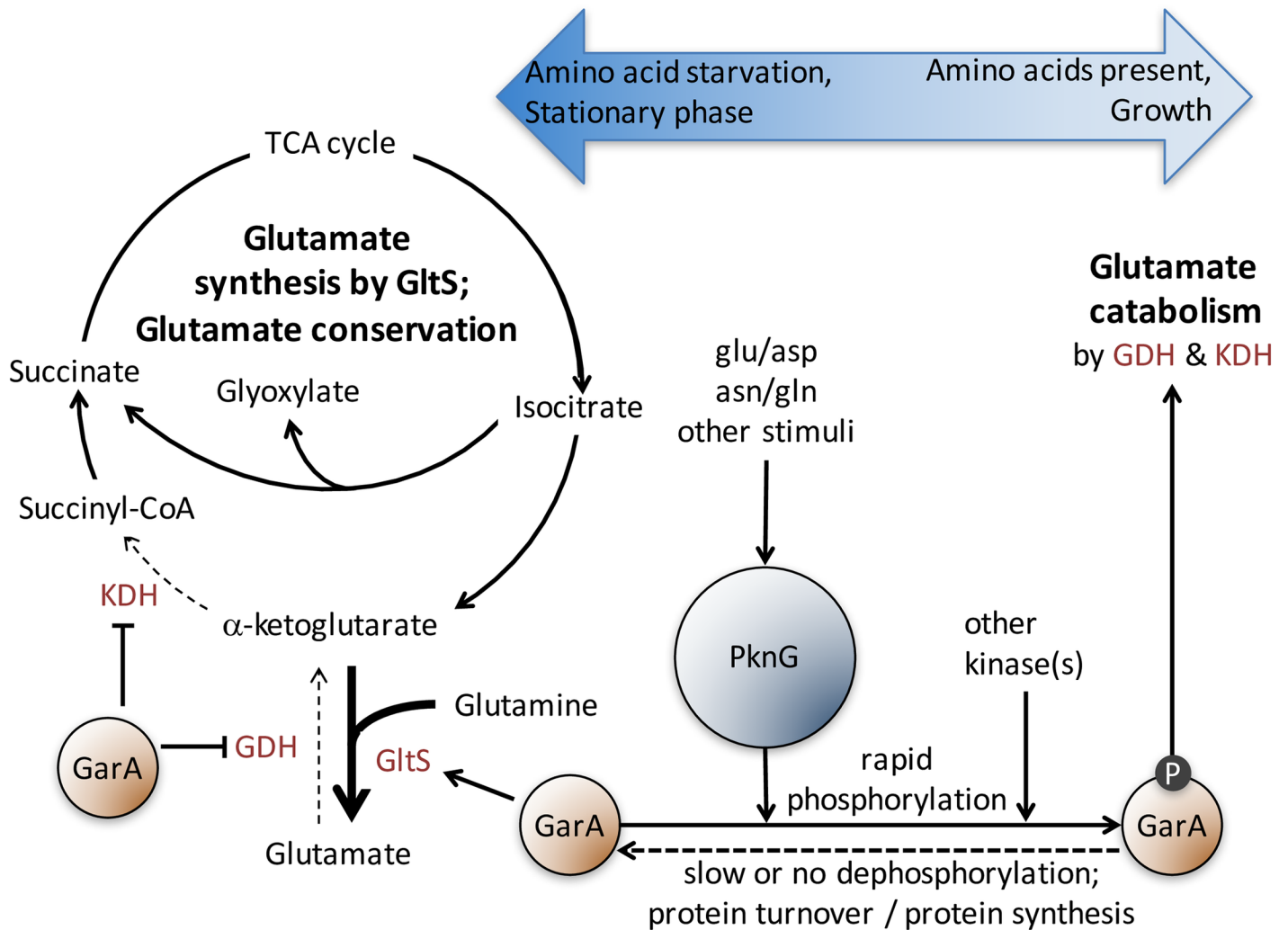
Fig 8. A model depicting control of the TCA cycle and glutamate metabolism by PknG and GarA. When PknG activity is low, unphosphorylated GarA activates glutamate synthesis and inhibits glutamate catabolism by direct binding to the relevant enzymes. When PknG activity is stimulated, for example by glutamate and aspartate, GarA become phosphorylated, causing a shift in metabolism towards glutamate catabolism. KDH is the alpha-ketoglutarate dehydrogenase complex, GDH is glutamate dehydrogenase, GltS is glutamate synthase.
