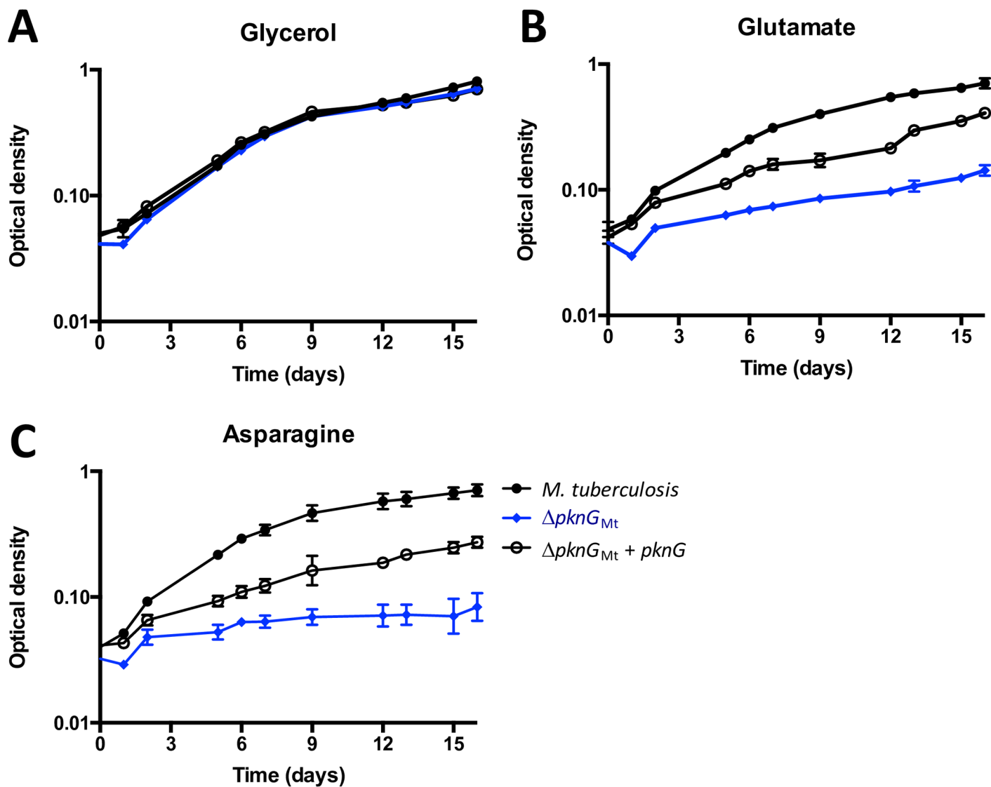
Fig 3. pknG disruption in M. tuberculosis caused a nutrient-dependent growth defect. (A) All strains grew at the same rate on minimal medium supplemented with glycerol 0.2%. \Delta pknG_{Mt} (blue diamonds) grew more slowly than wild type M. tuberculosis (black circles) when the sole carbon source was (B) glutamate 10 mM or (C) asparagine 10 mM. Plasmid-encoded PknG (empty circles) partially restored the growth defect. Graphs show the mean and standard deviation of three independent experiments.
