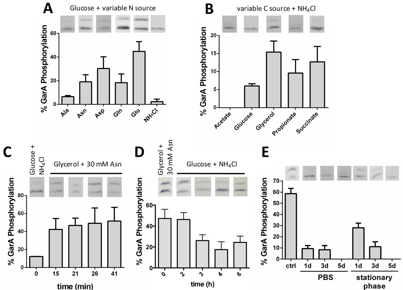
Fig 5. GarA phosphorylation in M. smegmatis was regulated by nutrient availability. The reporter strain of M. smegmatis was cultured in different media and cell lysates analysed by Western blot and densitometry. (A) Glutamate and related amino acids triggered phosphorylation of GarA: the nitrogen source is indicated and the carbon source was glucose. (B) The supplied carbon source affected phosphorylation of GarA: the carbon source is indicated and the nitrogen source was NH 4 Cl. (C) Phosphorylation of GarA occurred rapidly when cells were cultured in poor medium and then given supplementary nutrients (initially 1% glucose with 10 mM NH 4 Cl and 0.05% tyloxapol, then 1% v/v glycerol and 30 mM asparagine were added at time zero). (D) Dephosphorylation of GarA occurred slowly when cells switched from rich to poor medium (initially 1% glycerol with 30 mM asparagine and 0.05% Tween 80 then switched to 1% glucose with 10 mM NH 4 Cl and 0.05% tyloxapol). (E) GarA was predominantly unphosphorylated when M. smegmatis were in stationary phase or starved in PBS. The reporter strain of M. smegmatis was grown in Sauton's medium with shaking for 5 days. For the starvation experiment exponentially growing M. smegmatis were washed with PBS and incubated in PBS with 0.05% tyloxapol for 5 days. Values represent mean and standard deviation of at least three independent replicates.
