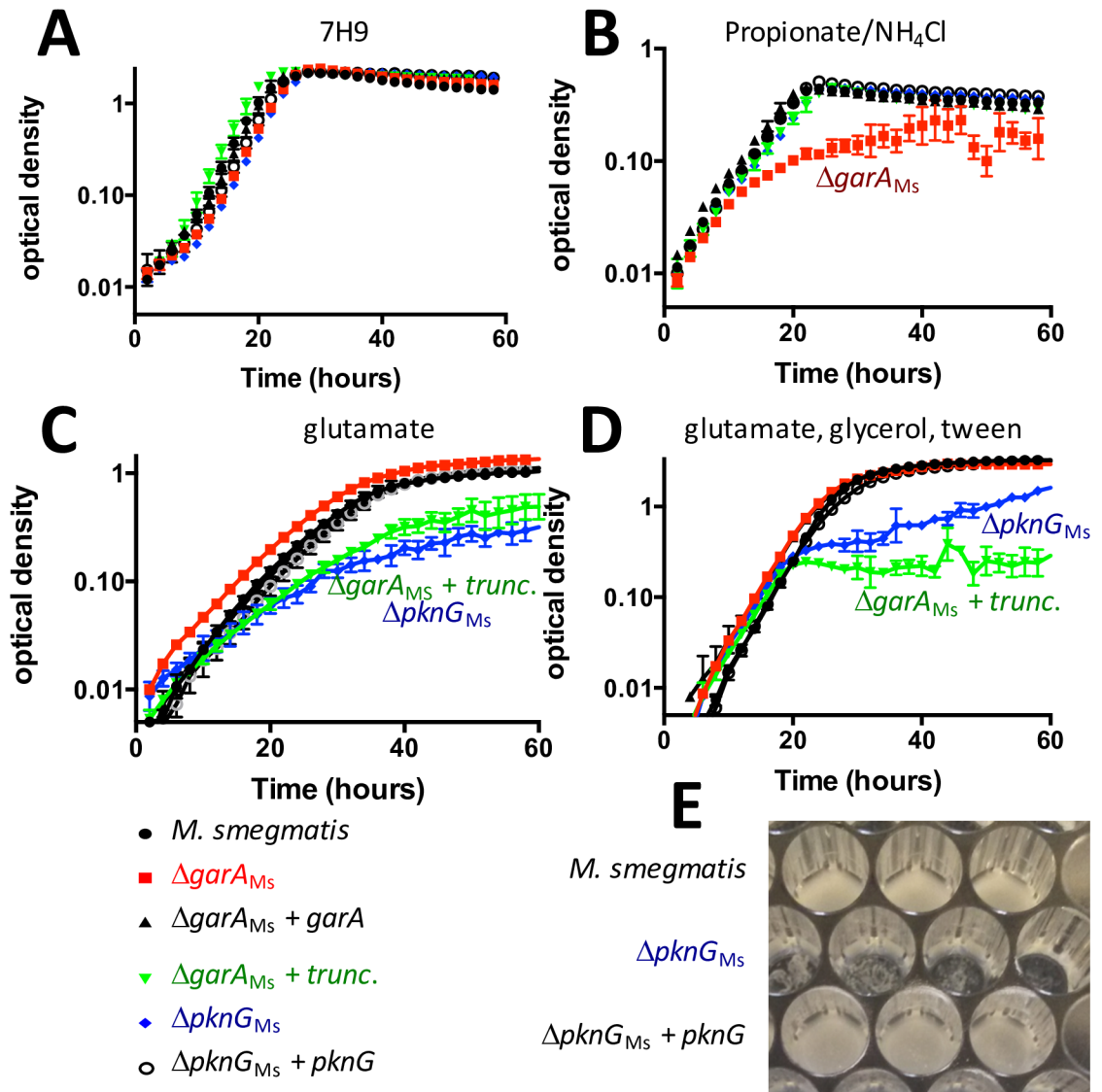
Fig 2. Disruption of pknG or removal of the phosphorylation motif of garA caused a nutrient-dependent growth defect in M. smegmatis . (A) All strains grew at the same rate on standard Middlebrook 7H9 medium. (B) \Delta garA_{Ms} grew slower than wild type on minimal Sauton's medium containing 20 mM propionate, 20 mM NH 4 Cl plus 0.05% tyloxapol, and this growth defect could be fully complemented by GarA lacking phosphorylation sites (truncated "trunc." garA ). (C + D) \Delta pknG_{Ms} grew slower than wild type and formed clumps (inset photo) on medium containing glutamate as sole carbon (C) or nitrogen source (D) (minimal Sauton's with either 30 mM glutamate plus tyloxapol, or 1% glycerol, 10 mM glutamate plus tyloxapol). Data plotted are the mean and standard deviation of at least 3 independent experiments. (E) \Delta pknG_{Ms} formed clumps when glutamate was the sole carbon or nitrogen source. The photograph shows a microplate from growth curve (D) imaged at 60 hours. Growth of \Delta garA_{Ms} complemented with phosphoablative GarA (EAAS) was equivalent to that of \Delta pknG_{Ms} complemented with truncated GarA in all tested conditions so only the dataset for truncated GarA is shown for clarity.
