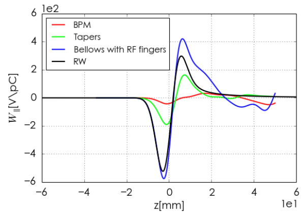
Figure 7: Longitudinal wake potentials for a 4mm Gaussian bunch given by RW, BPMs, tapers and bellows with RF fingers.
