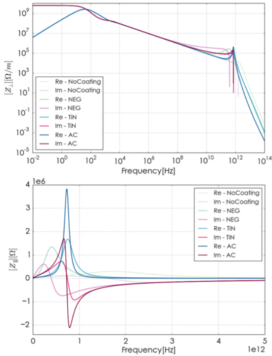
Figure 1: Real and imaginary part of the transverse (top) and longitudinal (bottom) RW impedances as a function of the frequency in the case of no coating, NEG coating, TiN coating and Carbon coating.
