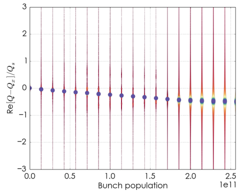
Figure 4: TMCI threshold evaluated with PyHEADTAIL by taking into account the bunch lengthening due to the longitudinal wake in the case of Carbon coating.
