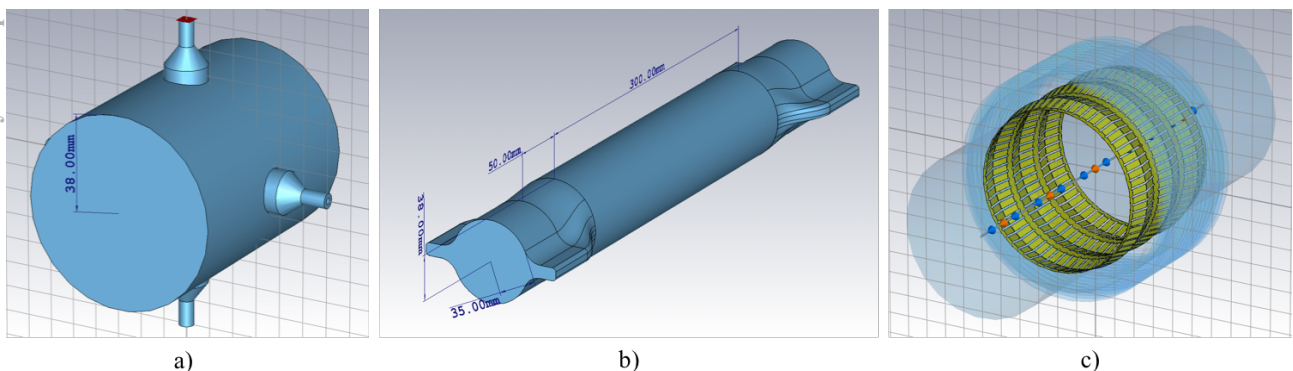
Figure 6: CST models of BPMs, tapers and bellows with RF fingers.
