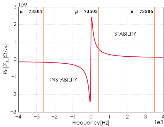
Figure 5: Coupled bunch spectrum and real part of the RW impedance in the case of no coating as a function of the frequency for the fractional tune \nu_\beta = 0.14 .
