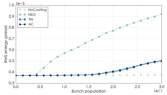
Figure 3: RMS energy spread as a function of the bunch intensity given by PyHEADTAIL by considering only the RW impedance in the case of no coating and NEG, TiN and AC coatings.
