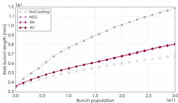
Figure 2: RMS bunch length as a function of the bunch intensity given by PyHEADTAIL by considering only the RW impedance in the case of no coating and NEG, TiN and AC coatings.
