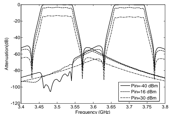
Fig. 10. Attenuation frequency dependence. Note that this corresponds to the transmission S_{21} term for each input power, P_{in} .
