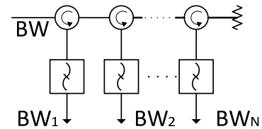
Fig. 6. Multiplexing architecture based on a Circulator-Coupled approach.
