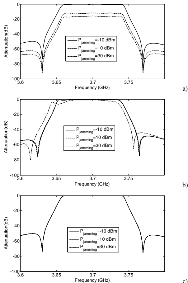
Fig. 11. Filter attenuation response ( S_{21} parameter) when a jamming signal of -10 dBm, 10 dBm and 30 dBm is set at the adjacent channel. a) SLS at the first resonator, b) SLS at the 3rd resonator and c) SLS at the last resonator.
