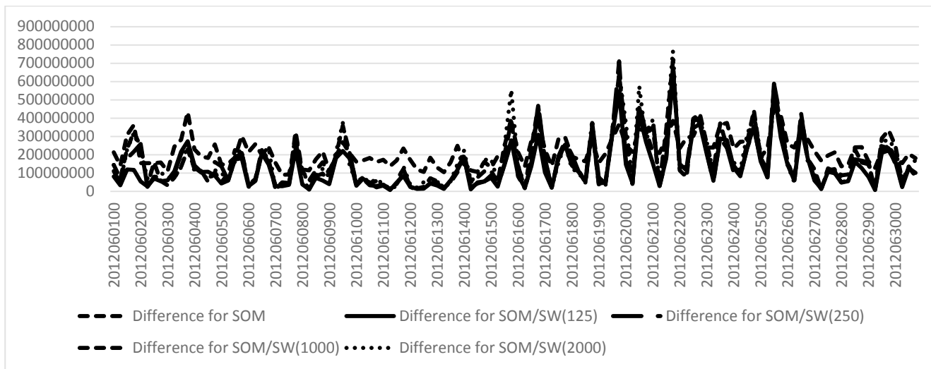
Figure 7 Graph depicts the comparison of the SOM and SOM+SW (with 4 different threshold values; 125 kB, 250 kB, 1000 kB, and 2000 kB)
