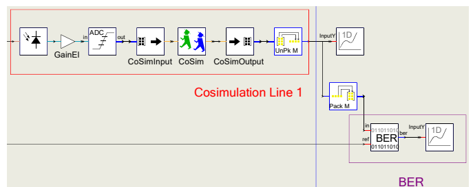
Fig. 4. Cosimulation line on receiver part and BER calculation
