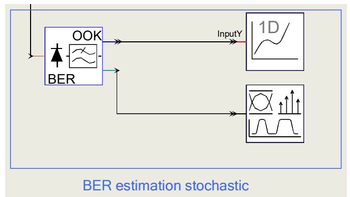
Fig. 3. BER estimation part
