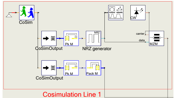
Fig. 2. Transmitter for NG-PON2 in cosimulation mode
