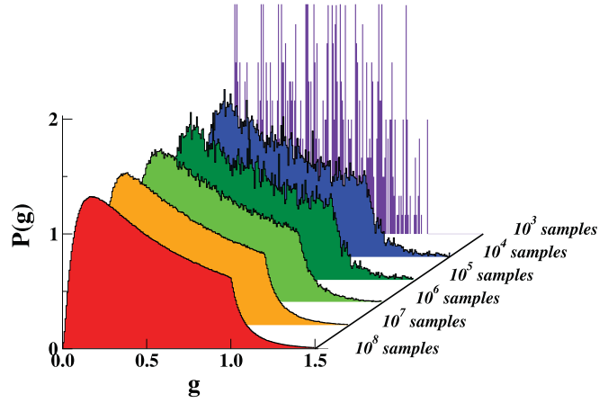
Fig. 54. Evolution of the conductance distribution with the number of MC steps (samples) for N = 5 for a converged value \langle g \rangle = 1/2 . The MC calculation is performed by using the JPD function [S21].
