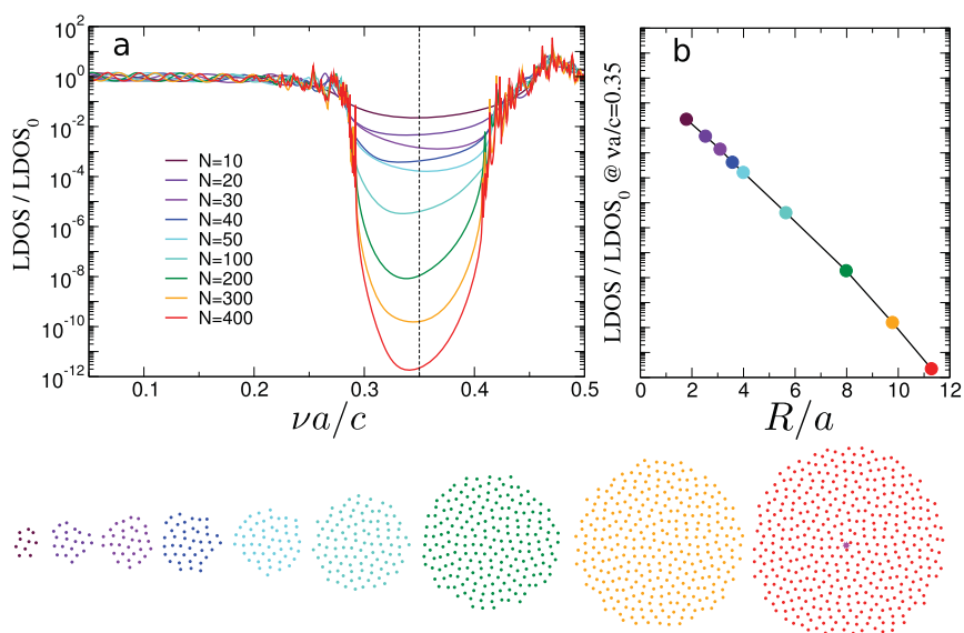
Fig. 57. (A) Local DOS, LDOS(r_e) , normalized to vacuum's LDOS ( LDOS_0 ) for a single finite sample with \chi = 0.40 as a function of the frequency \nu for different system sizes (total number of particles N ). The actual samples investigated are shown at the bottom and the central magenta colored point corresponds to r_e . (B) Normalized LDOS for a frequency \nu a/c = 0.35 inside the gap region, as a function of the system radius R/a (with N = \pi(R/a)^2 ).
