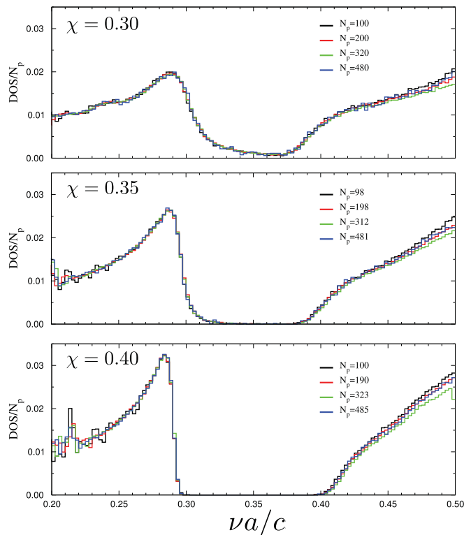
Fig. 56. DOS normalized by the number of rods (see text) for different sizes and stealthiness parameters in the region \chi \in [0.3, 0.4] where the PBG opens.
