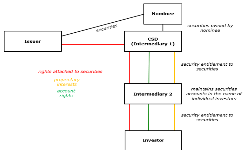
Diagram 48-1: Security entitlement model
