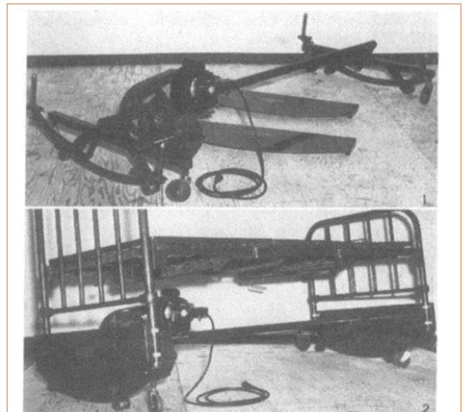
Fig. 1.—Mechanism of oscillatory bed support, including the two end shields, unattached. Fig. 2.—Standard (Simmons) hospital bed mounted on the oscillatory support with the end shields attached.
