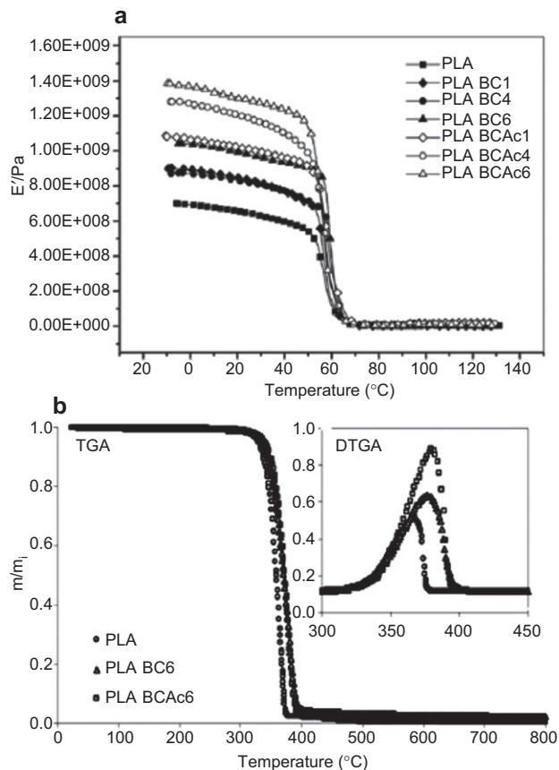
Figure 3 Properties of PLA and PLA-BC composites.
