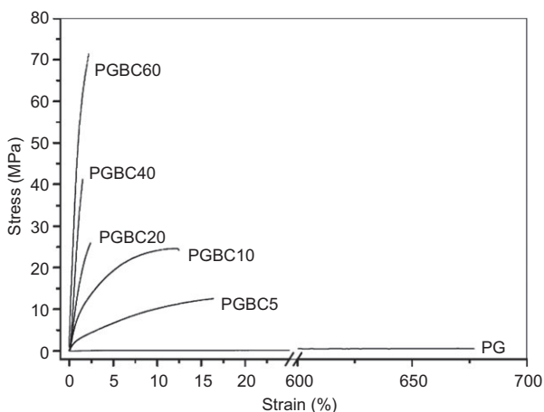
Figure 6 Stress-strain curves of PG and PG-BC nanocomposites (PGBC). The numbers indicate the BC concentration in %.
