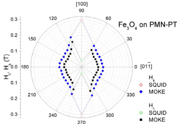
FIG. 2. (Color online) Angular dependence of the coercive field H_c and switching field H_s , deduced from MOKE and SQUID loops of the \text{Fe}_3\text{O}_4 film on (01\bar{1}) PMN-PT, showing a [100] hard axis. The line is a guide to the eye.
