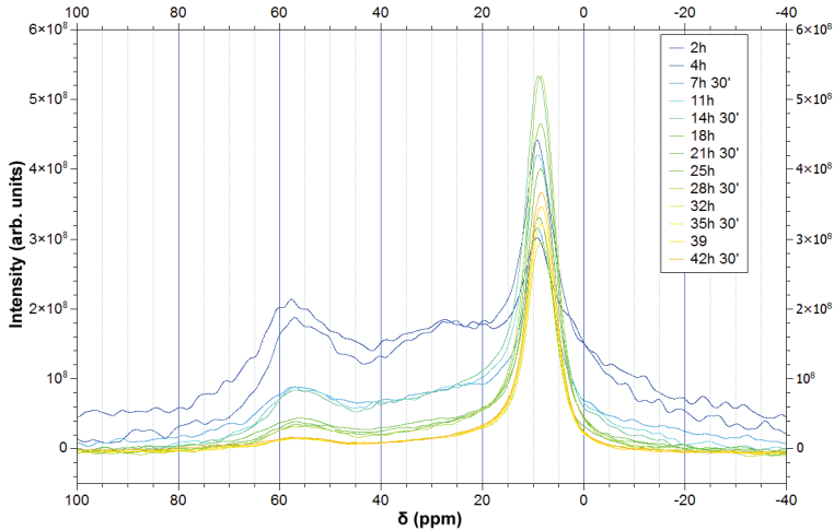
FIG. 12. ^{27}\text{Al} NMR spectra of MK mixed with lime over a period of time of 42 h and 30 minutes at 30^\circ\text{C} temperature.
