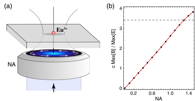
FIG. 3 (color online). (a) Illustration of the experiment. A spatially isolated Eu^{3+}:Y_2O_3 nanoparticle is excited by an azimuthally polarized beam (the arrows show the direction of electric field vector) focused by a 1.3 NA objective lens. The same lens is used to collect spontaneously emitted photons from the nanoparticle. (b) Ratio of the maximum magnetic field strength (center of beam) to the maximum electric field strength (outer ring) of an azimuthally polarized laser beam as a function of the numerical aperture. The field strengths were evaluated just above a glass air interface. The horizontal dashed line indicates the ratio for NA = 1.3 used in our experiments.
