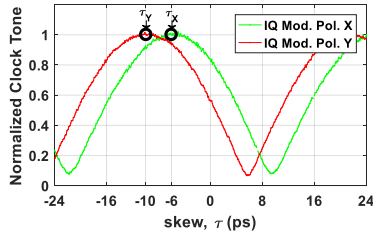
Fig. 5: Experimental curves for clock tone relative to transmitter time skew in a single-polarization signal.
