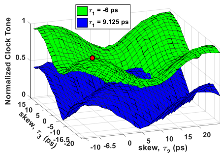
Fig. 6: Experimental curves for clock tone relative to transmitter time skew in a dual-polarization signal.
