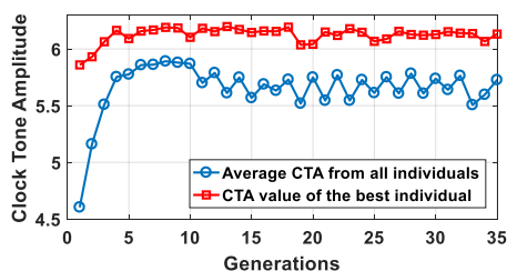
Fig. 7: Experimental CTA evolution for the proposed GA-based time skew estimator.
