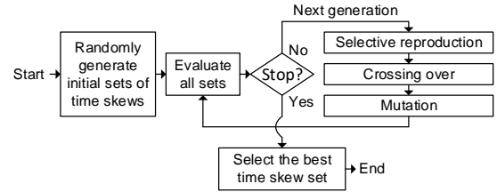
Fig. 3: Genetic algorithm block diagram.
