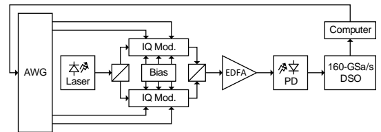
Fig. 4: Experimental setup.
