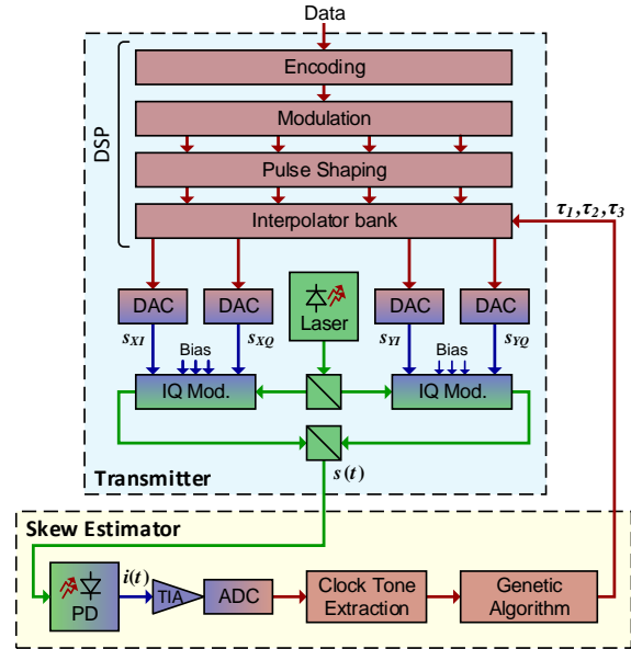
Fig. 1: Proposed algorithm scheme.
