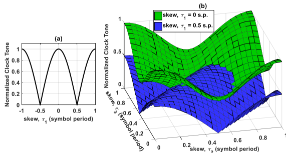
Fig. 2: Theoretical curves for CTA relative to transmitter time skew for (a) single-polarization signal; (b) dual-pol. signal.
