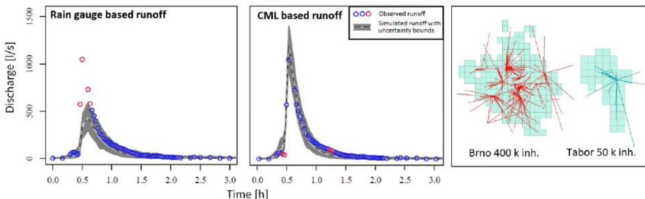
Fig. 1 – Left and middle: Runoff simulated based on three rain gauges about 2.5 km from the catchment located in Prague (CZ) in comparison to the runoff simulated from CMLs. Blue circles depict observed runoff inside of uncertainty bounds whereas red circles are outside of them. Right: CML topology in a city with 50 and 400 thousand inhabitants.
