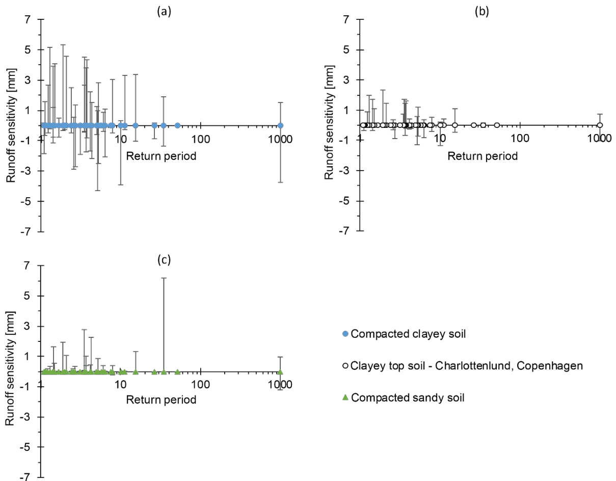
Fig. 4. Difference between runoff simulated in continuous simulations ( Q_{tot,acc} ) and assuming initial conditions as maximum ( Q_{tot,min} ) or minimum ( Q_{tot,max} ) infiltration capacity for historical rain events. Positive values correspond to Q_{tot,max} - Q_{tot,acc} , negative values to Q_{tot,acc} - Q_{tot,min} . Subfigures show results for (a) compacted clayey soil, (b) clayey top soil and (c) compacted sandy soil.
