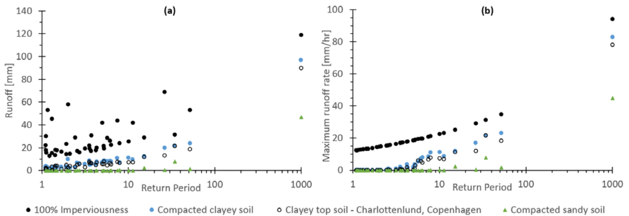
Fig. 3. (a) Simulated total runoff depth for historical rain events with return periods based on the maximum hourly rain intensity. There is no simulated runoff from non-compacted sandy soils. (b) Simulated maximum hourly runoff rate for the same historical rain events.
