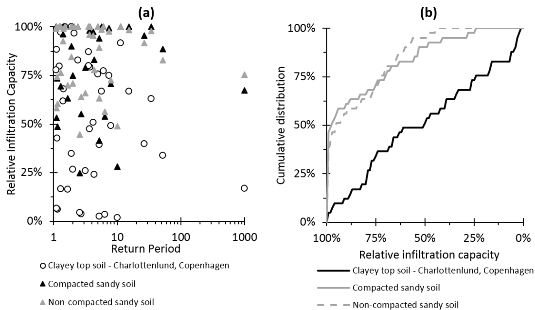
Fig. 2. (a) Relative infiltration capacity at start of large rain events for sandy and clayey soils for events with different return periods. (b) Cumulative distribution of the relative infiltration capacity in (a).
