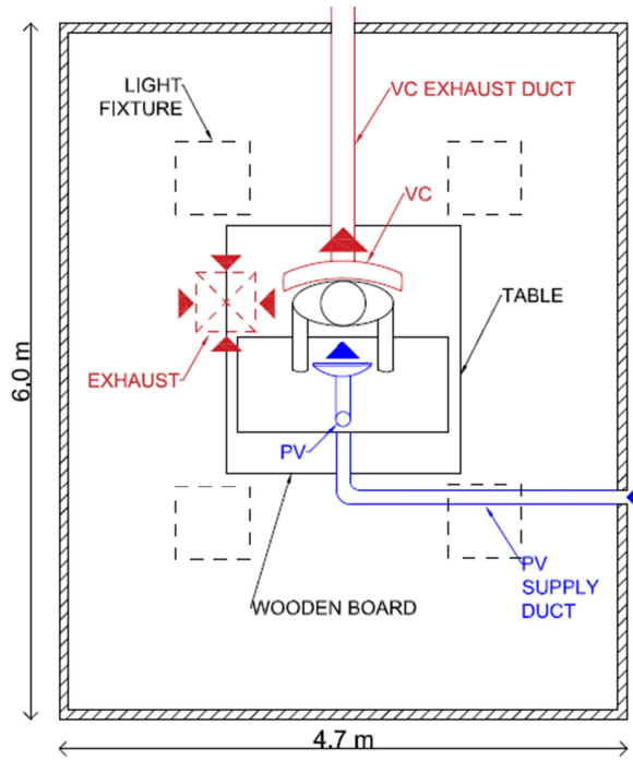
Figure 1: Experimental set-up in the climate chamber.
