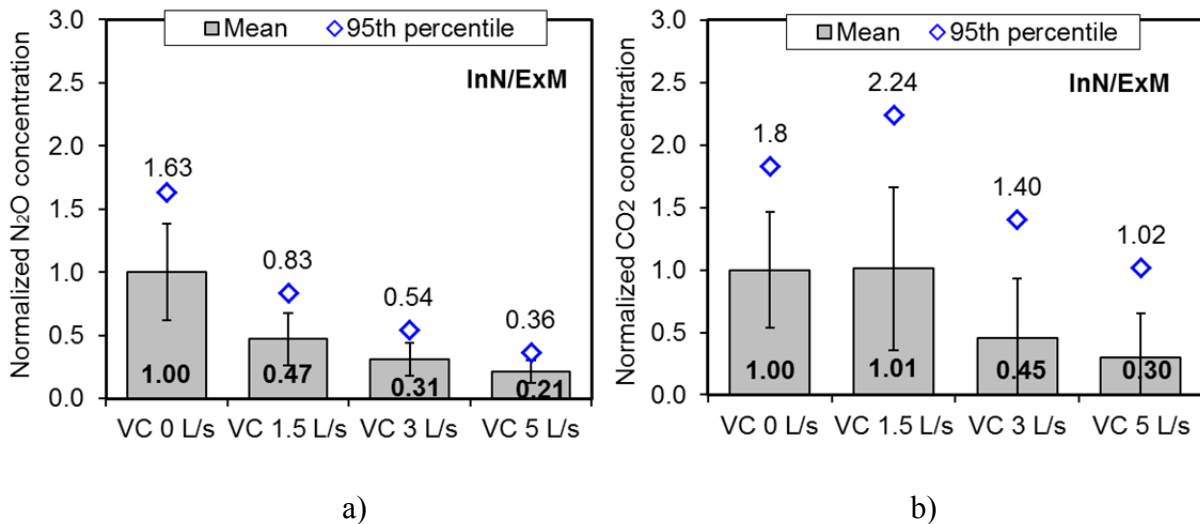
Fig. 7. a) Normalized mean and 95 th percentile of N 2 O concentration (pollution from the groins) and b) Normalized mean and 95 th percentile of excess CO 2 concentration (pollution from the armpits). The error bars show the normalized standard deviation.
