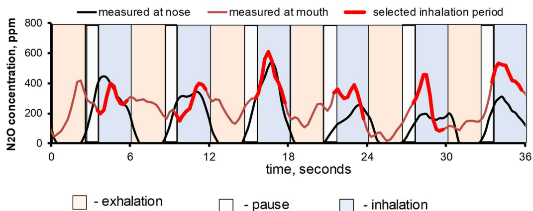
Figure 4: An example of the binary signal for the breathing mode inhalation mouth/exhalation nose/pause obtained from the measured instantaneous N_2O concentrations at the mouth and at the nose. The selected concentrations during the inhalation are marked with red.
