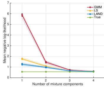
Figure 4: The mean negative log-likelihood experiment.
