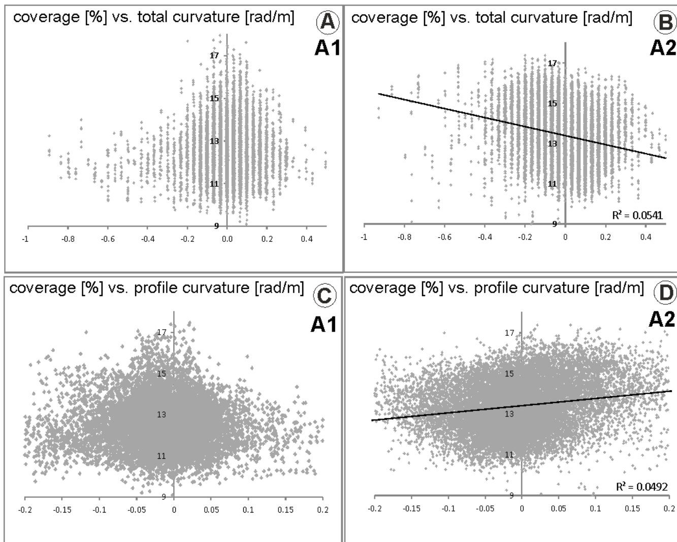
Figure A1. Scatterplots indicating the relation between Mn-nodule coverage and total curvature (A,B) and profile curvature (C,D) in the A1 and A2 sub-areas. Only in area A2 weak correlations could be observed.
