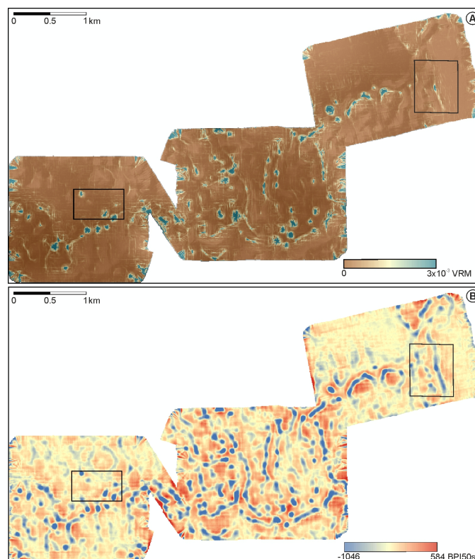
Figure A3. A) Terrain Roughness-indicating map derived from AUV-acquired bathymetry data (calculated with the VRM algorithm Sappington et al. (2007)). B) BPI50st derived from the AUV-obtained bathymetric data set; the lowest values indicate areas with 'pit-structures' that are observed throughout the entire area.
