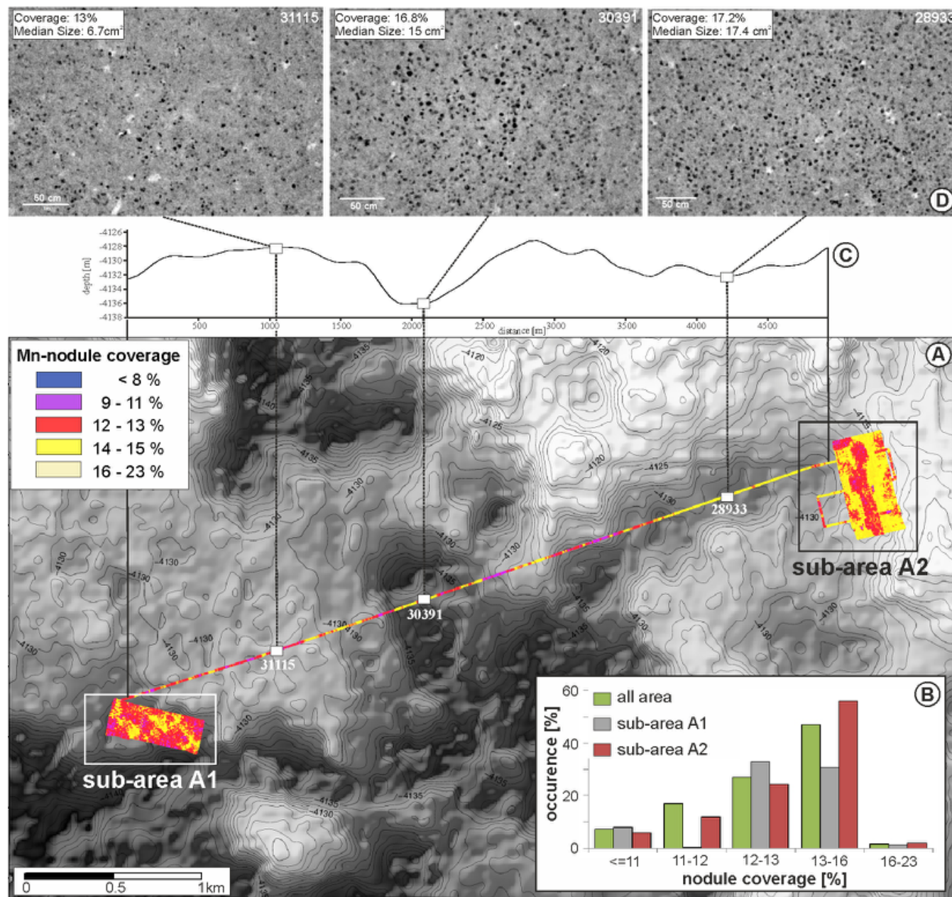
Figure 5. A) Bathymetric map (ship-based MBES) of the Working Area with nodule coverage calculated from AUV photo survey; the photo examples in D) show the Mn-nodule coverage and median size in different areas. B) Statistical evaluation of nodule coverage for the entire photo survey (green bars; 30,038 photos) and the sub-areas A1 (gray bars; 10,120 photos) and A2 (red bars; 16,890 photos).
