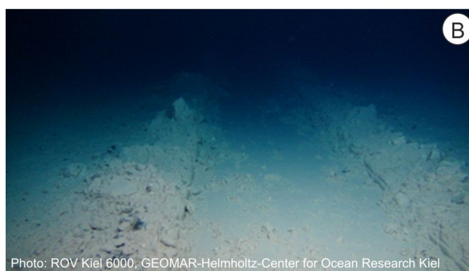
Figure A2. A) The Epibenthic sled that created the monitored sediment plume (Photo: A. Hilario) Brenke (2005). B) Track created by the EBS at the seafloor, approximately 20 cm deep and 1.5 m wide Photo: ROV Kiel 6000, GEOMAR Helmholtz-Center for Ocean Research Kiel.
