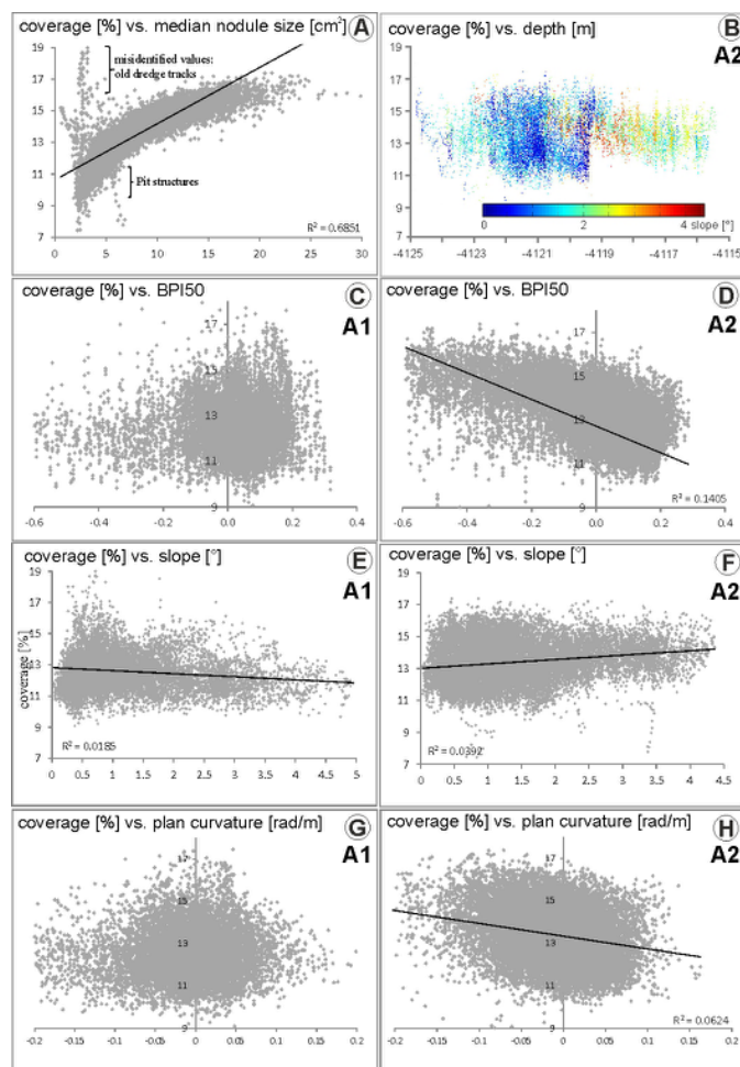
Figure 6. Scatter Plots indicating relationships between Mn-nodule percent coverage (%) and eight other nodule and terrain values: median nodule size in cm 2 (A), depth within the A2 sub-area (B, color-coded by slope), BPI50 (C,D), slope (E,F) and plan curvature (G,H). Charts (C,E,G) relate to sub-area A1; charts (B,D,F,H) to sub-area A2. The sub-areas show different correlations.
