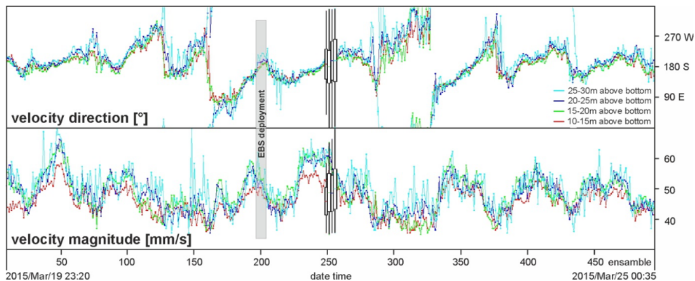
Figure A4. ADCP data obtained by while a DOS lander deployment during SO239 indicating a SSW current flow while the EBS deployment (grey shaded box; ensemble 196 to 204). Box plots show the mean and standard deviation of the time series of the entire deployment. Mean currents between 10 and 30 m above the bottom are towards the south with about 50 mm/s.
