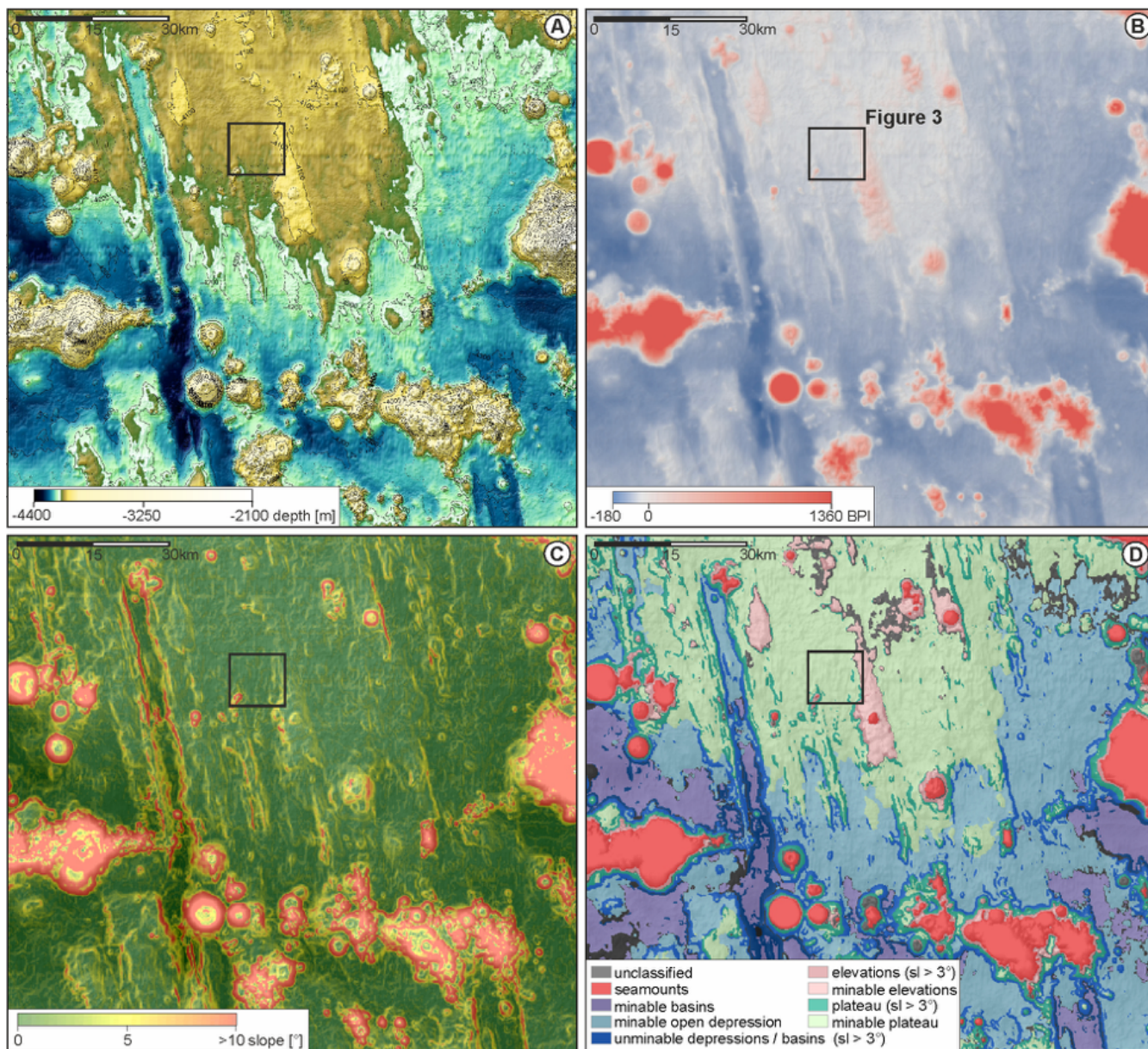
Figure 2. Overview maps of PA 1 showing A: Bathymetry, B: Bottom Positioning Index (BPI) with scalefactor 11,000 (grid cell size: 110m, inner radius: 10 cells, outer radius: 100 cells), C: Slope and D: Classification of the terrain based on the classification dictionary in Appendix Table A2 (sl = slope). Black squares mark the study area shown in Figure 3.
