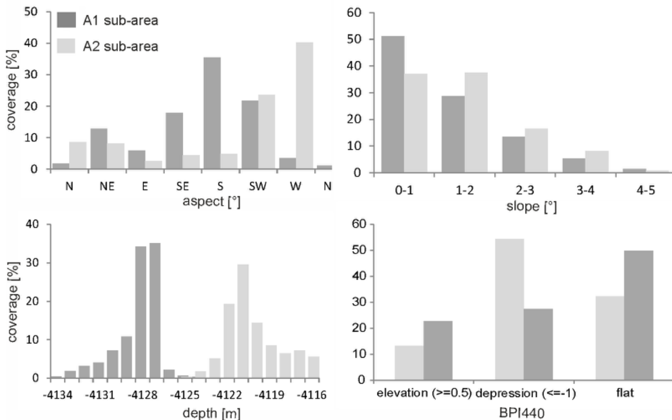
Figure 8. Distribution of derivative values in sub-area A1 and A2.
