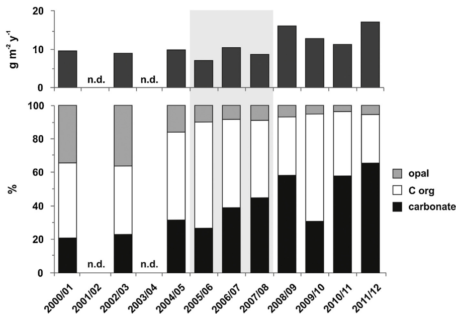
Fig. 6. Annual flux of biogenic matter (top) and percentage composition of its components (bottom) between 2000 and 2012 (n.d. = no data). The gray-shaded area indicates the period of the WWA.
