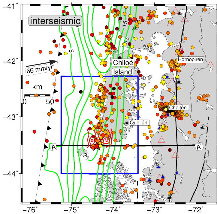
Figure 6: The 2016 Chiloé earthquake and interseismic activity in the region of Chiloé Island. Circles indicate interseismic activity (CSN catalogue, 01/01/2008 until 24/12/2016 and seismicity from Lange et al., 2007) together with the slip model of the 1960 Valdivia earthquake based on the inversion of land-level changes (Moreno et al., 2009) shown with green lines (5 m slip contours). Red lines indicate the 1 m slip contours of the 2016 Chiloé earthquake. Volcanoes are indicated with red triangles. Black (CSN) and blue (Sernageomin) triangles indicate local seismic stations used in this study. Blue box indicates location of figure 4. The location of the profiles shown in figures 6 and 7 are shown with a black line and labelled with A-A'.
