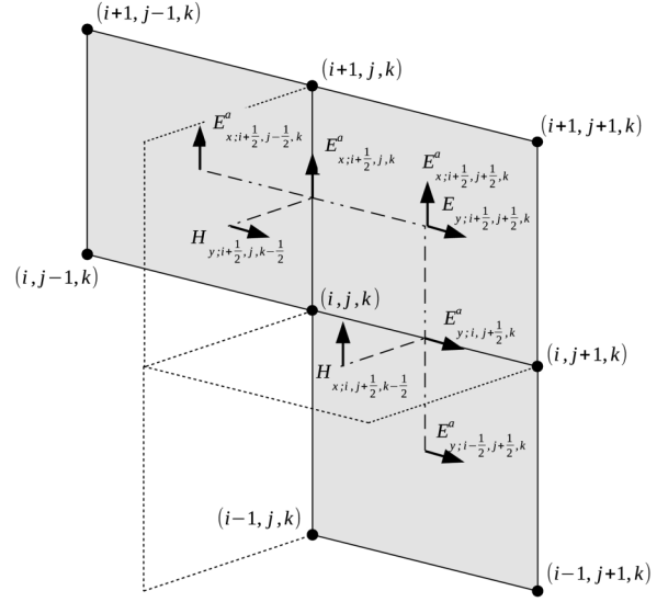
Fig. 4. Spatial interpolation of the tangential electric fields on the SIBC faces (shaded) for the tangential magnetic field updates adjacent to the SIBC on the z -low side of a z -normal face.
