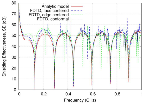
Fig. 9. Shielding effectiveness at the center of the hollow spherical shell with \sigma = 1 kS/m and thickness h = 1 mm comparing the analytic solution to the different FDTD methods.
