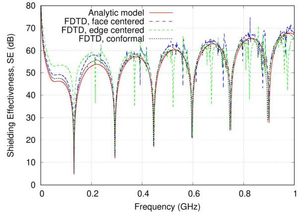
Fig. 10. Shielding effectiveness at the center of the hollow spherical shell with \sigma = 200 S/m and thickness h = 5 mm comparing the analytic solution to the different FDTD methods.
