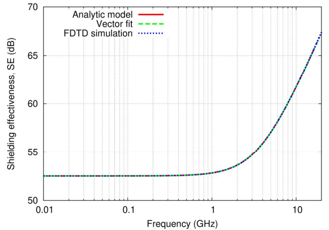
Fig. 6. Shielding effectiveness of an isotropic metalized fabric.
