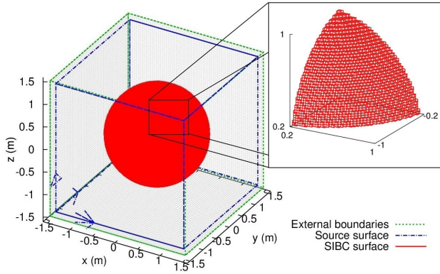
Fig. 8. Geometry of the hollow spherical shell test-case. The shell radius is 1 m and it is illuminated by a y -polarized plane-wave propagating along the x -direction generated by a total-field scattered field boundary.
