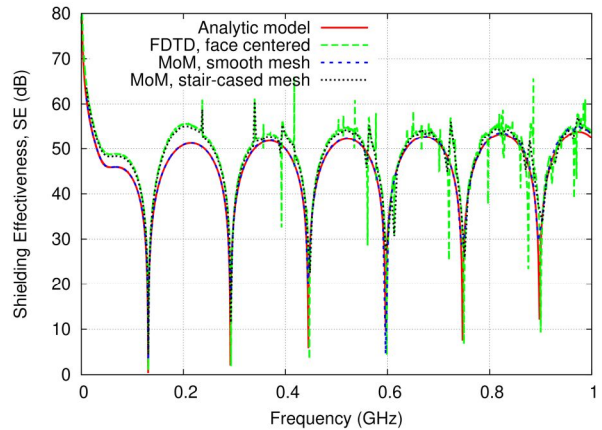
Fig. 11. Shielding effectiveness of the hollow spherical shell with \sigma = 1 kS/m and thickness h = 1 mm showing MoM results with smooth and stair-cased meshes compared to the analytic model and face centered FDTD results.
