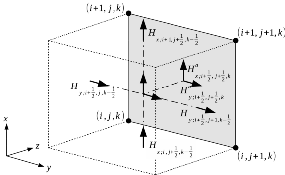
Fig. 3. Spatial interpolation of the tangential magnetic fields to the SIBC face centers for the electric field update on the z -low side of the z -normal face centered on (i+1/2, j+1/2, k) . The SIBC face is shaded.
