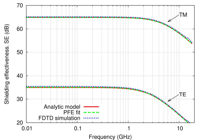
Fig. 7. Shielding effectiveness of an anisotropic wire mesh.
