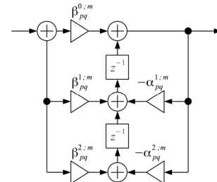
Fig. 2. The m -th direct-form-II-transpose second-order filter section of the SOS cascade for impedance matrix element Z_{pq} .
