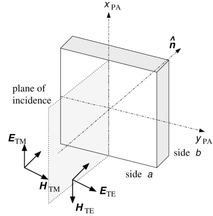
Fig. 1. Reflection and transmission of TM and TE polarized waves from a plane boundary in the principal axis coordinate system of the material's impedance matrix.
