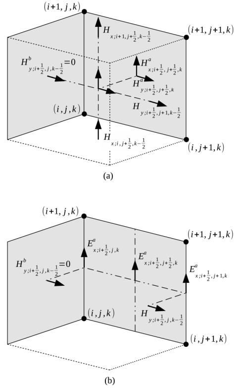
Fig. 5. Intersection between two SIBC faces (shaded) in the face centric approach showing the fields involved in: (a) The tangential magnetic field update adjacent to the SIBC; (b) The tangential electric field update on the SIBC.
