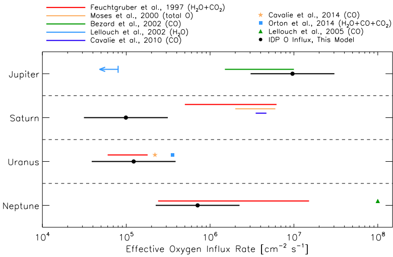
Fig. 6 A comparison of effective molecular oxygen influx rates to each of the giant planets from interplanetary dust grains (black) to various observational constraints (colour lines and points) (adapted from Poppe 2016)
