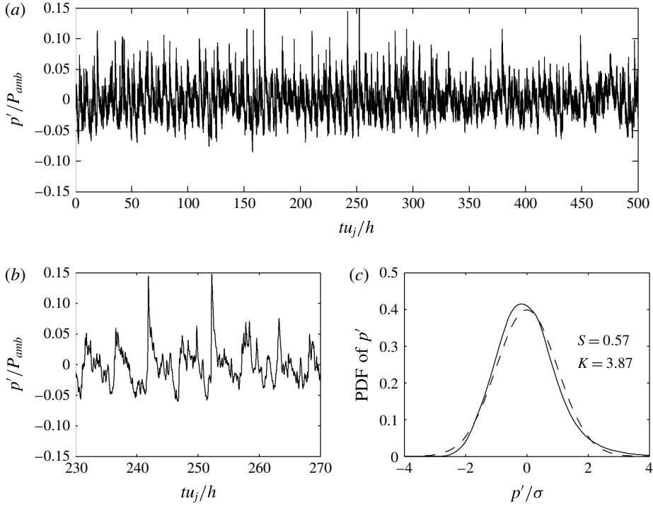
FIGURE 11. Pressure fluctuations at x=0 and y=8.5h for JetL5.5: (a) time variations over the entire simulation, (b) variations over a short period and (c) — probability density function and --- probability density function of a Gaussian distribution where \sigma represents the standard deviation of p' .
