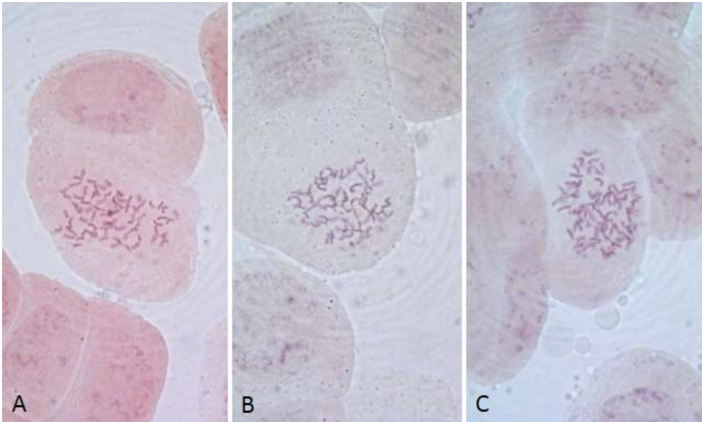
Fig. 10. Chromosome number of the triploid Hedera taxa: H. × soroksarensis ('Negro') (A), H. × schmidtii . (B) and H. × soroksarensis ('Woerner') (C). Cytological features were recorded using a 40× objective (magnification of 400× (A, B, C) in an optical microscope. Photo credit: Pintér I. and Lengyel Sz. (PINTÉR ined.).
