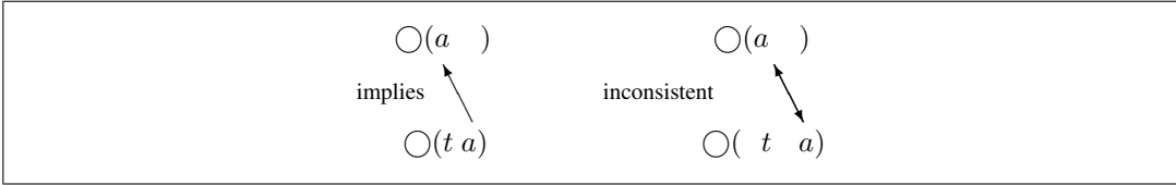
Figure 7: \bigcirc(t|a) is an ATD of \bigcirc(a|T) and \bigcirc(-t|\neg a) is a CTD of \bigcirc(a|T)
