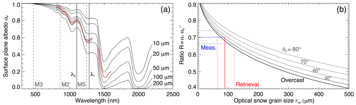
Figure 4. (a) Surface plane albedo for optical snow grain sizes between 10 and 200 \mu\text{m} ; \theta_0 = 54^\circ and A = 5.8 ( \chi data from Warren and Brandt, 2008). M3, M2, and M5 mark MODIS spectral bands used within the SGSP algorithm. \lambda_1 and \lambda_2 denote wavelengths used within the CORAS and SMART grain size retrieval. The red solid line and shaded gray show a spectral albedo measured by CORAS on 24 December 2013 (14:00 UTC). (b) Illustration of retrieval principle. Dependence of ratio \mathcal{R} with respect to optical snow grain size for different solar zenith angles (50 to 80^\circ ) and for overcast conditions; A = 5.8 ( \chi data from Warren and Brandt, 2008). Blue and red lines illustrate the retrieval of optical snow grain size from a measured albedo ratio \mathcal{R} = 0.7 with a relative uncertainty of 5.5 %.
