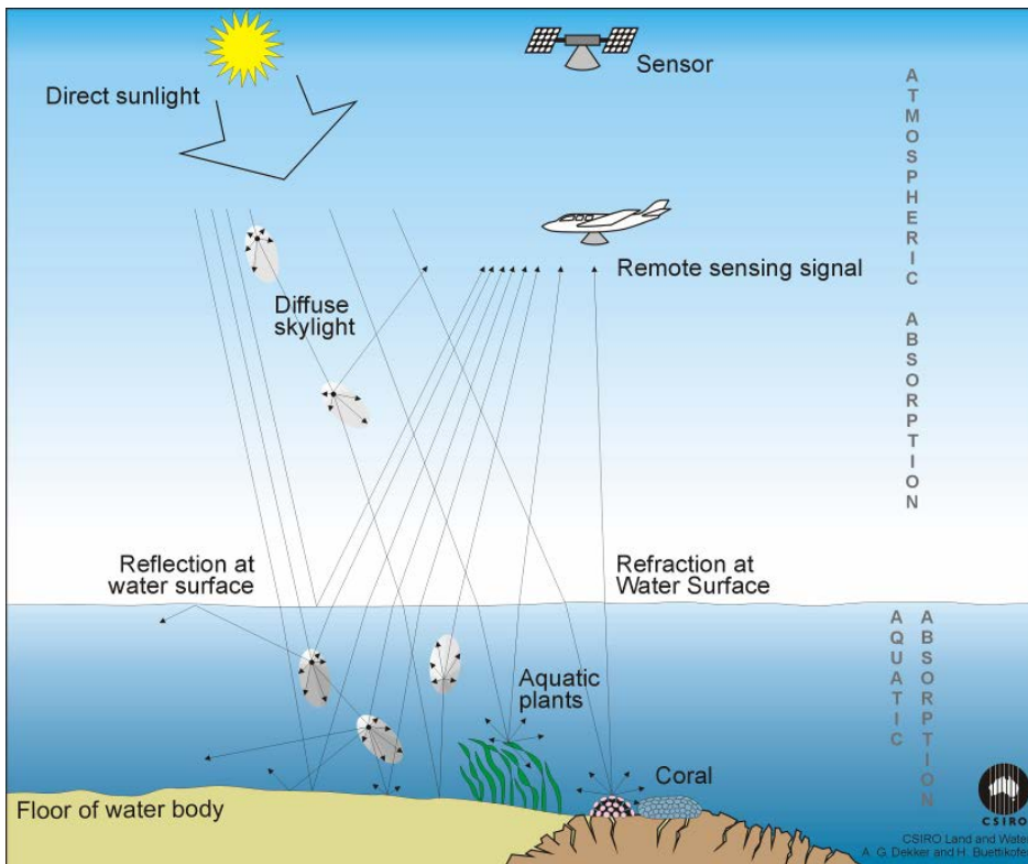
Figure 1.5 Schematic of the light Interactions that drive optical EO involving the air, water, and substrate
