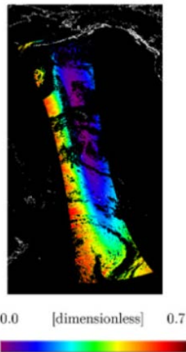
Figure 3.3 (after Meister et al., 2011) Degree of linear polarization (a dimensionless quantity from 0 to 1, where 0 is unpolarised light and 1 is completely linear polarised light) of the TOA radiances for an orbit of MODIS Aqua data over the Pacific Ocean for August 14, 2000. MODIS Aqua equator crossing time is 13:30; for a sensor with a noon crossing time a more symmetric distribution around nadir is expected.
