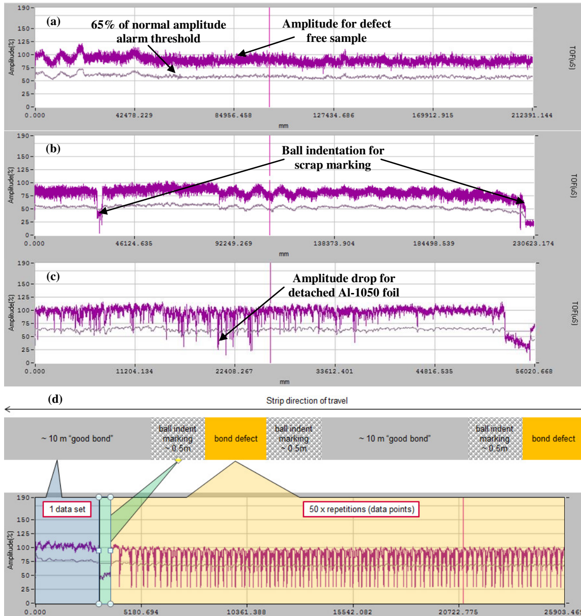
Figure 10. Results-based illustration of A-scan maximum amplitude trace: (a) SP1-R1 320 m, (b) SP2-R2 390 m, (c) SP3-D 80 m strips, (d) AD samples
