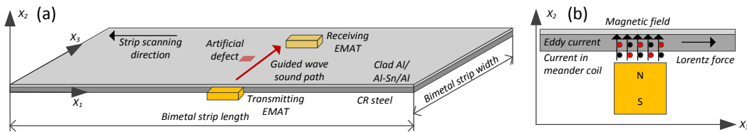
Figure 4. EMAT transducers to generate and receive guided waves in plates: (a) sound path, (b) interaction with material
