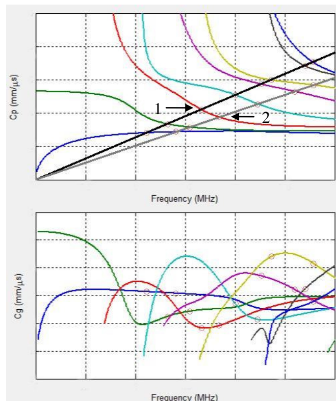
Figure 5. Dispersion curves of the four layer structure: (a) phase velocity with employed wave mode, (b) group velocity
