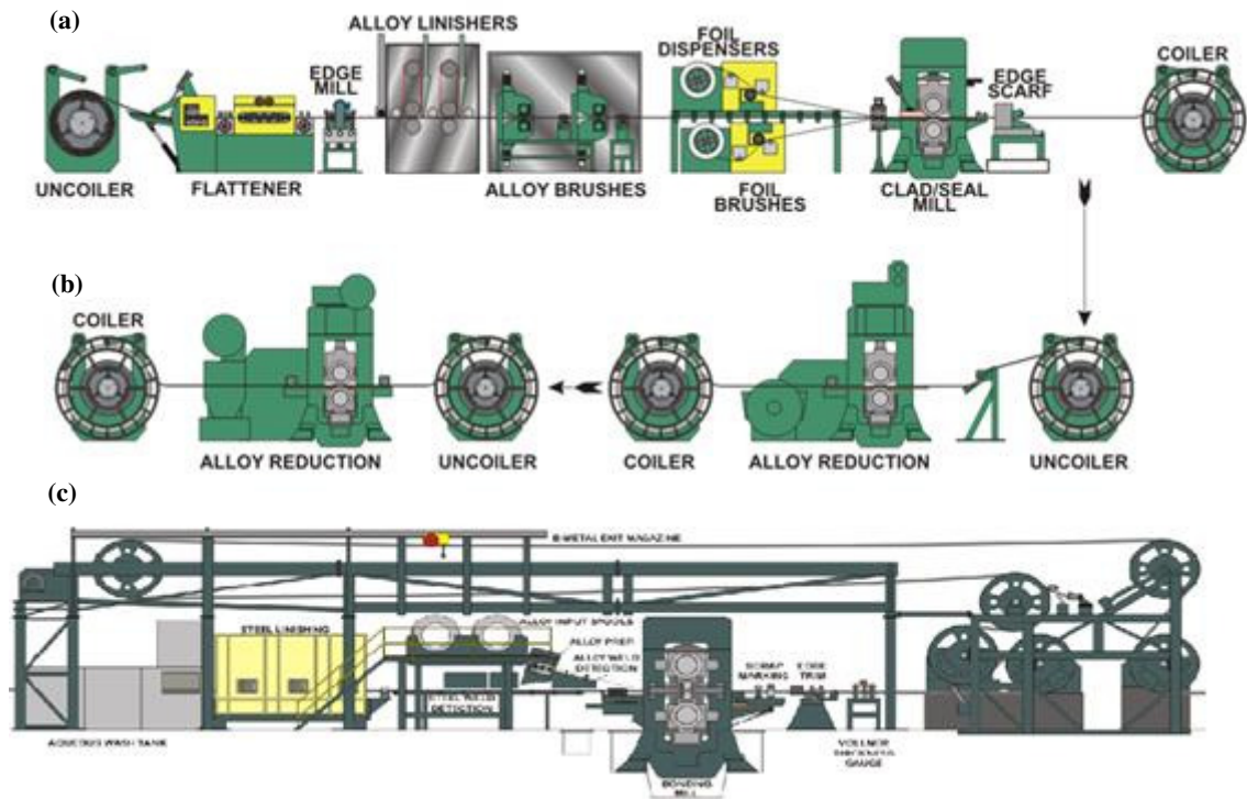
Figure 7. Al/Al-Sn/Al production process: (a) Al/Al-Sn/Al cladding, (b) clad Al rolling, (c) CRB of clad Al to steel
