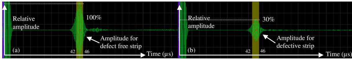
Figure 6. A-scan for (a) defect free and (b) defective Al/Al-Sn/Al/steel plate
