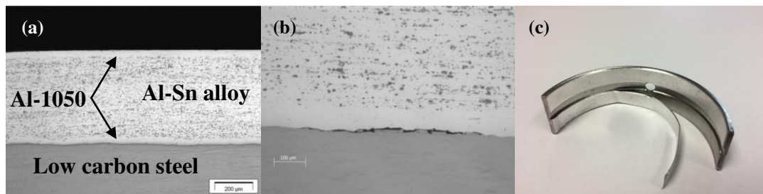
Figure 1. (a) Micrograph of the four-layered Al/Al-Sn/Al/steel structure with good bond, (b) delamination between Al-1050 and steel, (c) half shell bearing delamination
