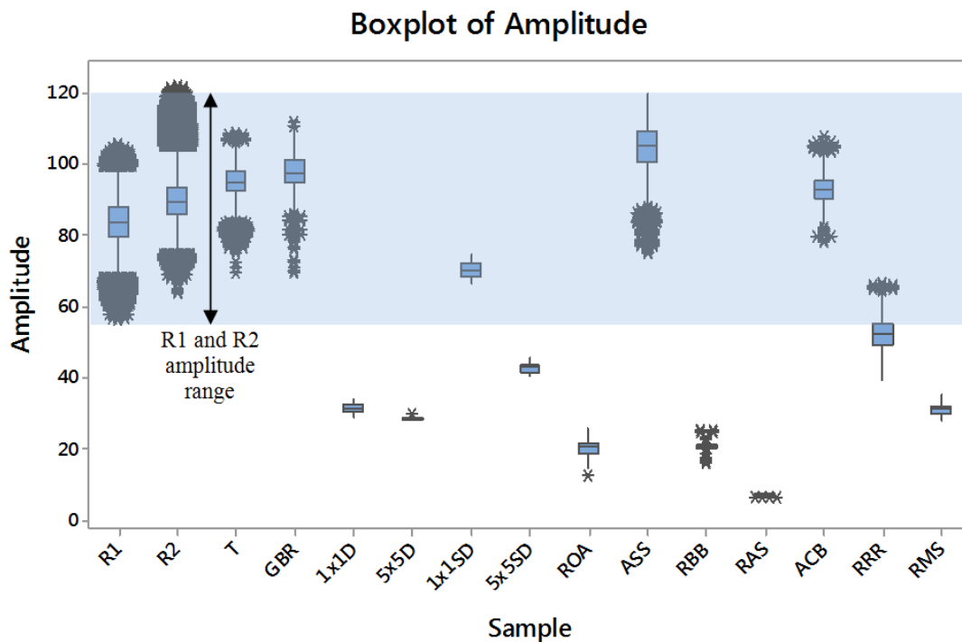
Figure 11. Boxplot of SP-R1, SP-R2 and AD strip samples showing central tendency and variability
