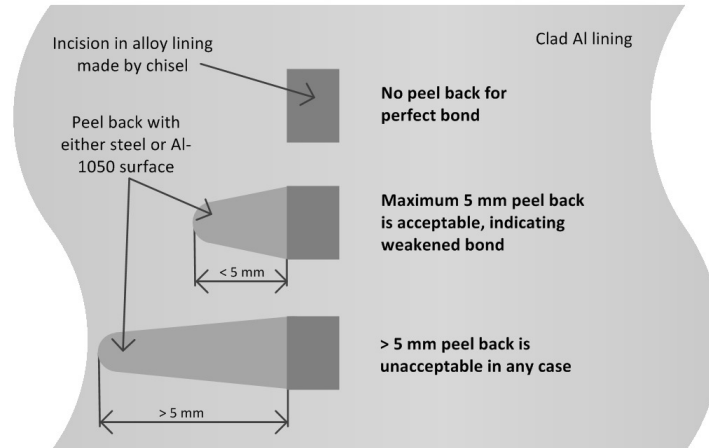
Figure 9. Clad Al lining adhesion peel back test procedure and pass/fail ratings
