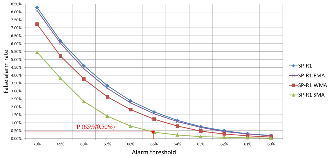
Figure 13. Relationship between false alarm rate and threshold for defect-free sample SP-R1
