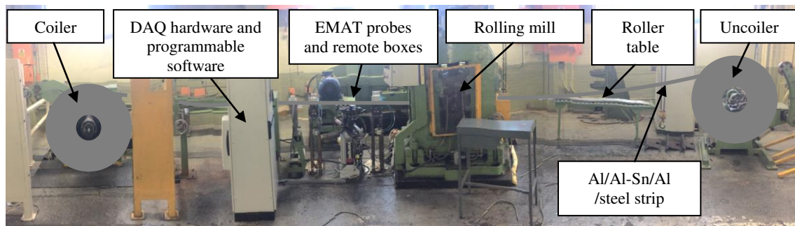
Figure 2. EMAT prototype inspection line for Al/Al-Sn/Al/steel strips
