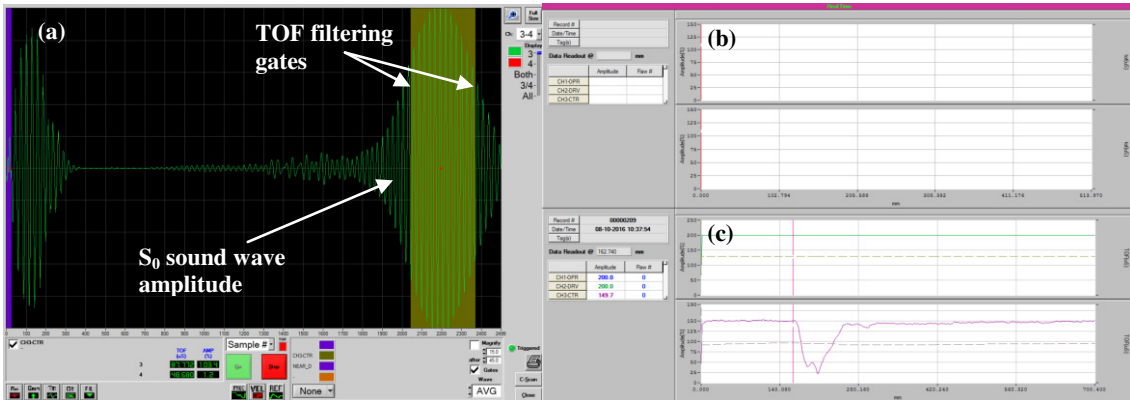
Figure 3. Temate® software a) A-scan oscilloscope, b) on-line A-scan maximum amplitude trace, c) A-scan maximum amplitude recall panel
