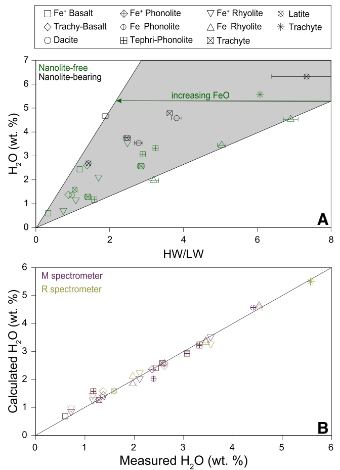
Fig. 9. A) Data from M spectrometer. Sample water content versus the HW/LW band area ratio calculated following the baseline protocol reported in this study. For each sample series, a linear relationship is observed when nanolite-free samples (green symbols) are considered. Nanolite-bearing samples (black symbols) do not follow such a trend. B) Data from both spectrometers. Comparison between measured and calculated water contents using Eq. (4) and parameters in Table 2. (For interpretation of the references to colour in this figure legend, the reader is referred to the web version of this article.)
