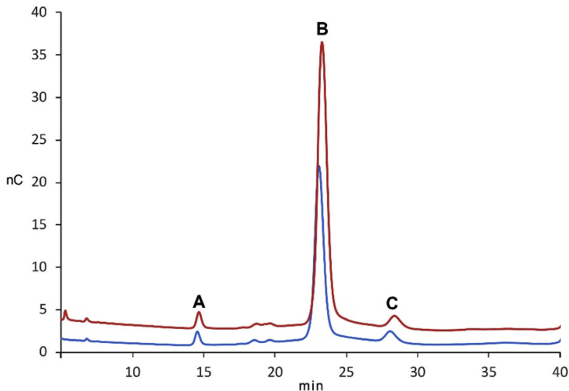
Fig. 2. Monosaccharide analysis of B. thailandensis E555:: wbl (pKnock-KmR) CPS by HPAE-PAD on Dionex Carbopac PA 20 column. The bottom trace shows the ion chromatogram of CPC hydrolysis products and the top one is the same sample spiked with 25 \mu M 6-deoxy-D-manno-heptose standard. Peaks correspond to (A) – unidentified sugar, (B)–6-deoxy-D-manno-heptose, and (C) – mannose. The analysis was performed on Dionex Carbopac PA 20 column (3 \times 150 mm) at 0.25 mL/min in 8 mM NaOH at 25 ^{\circ} C.
