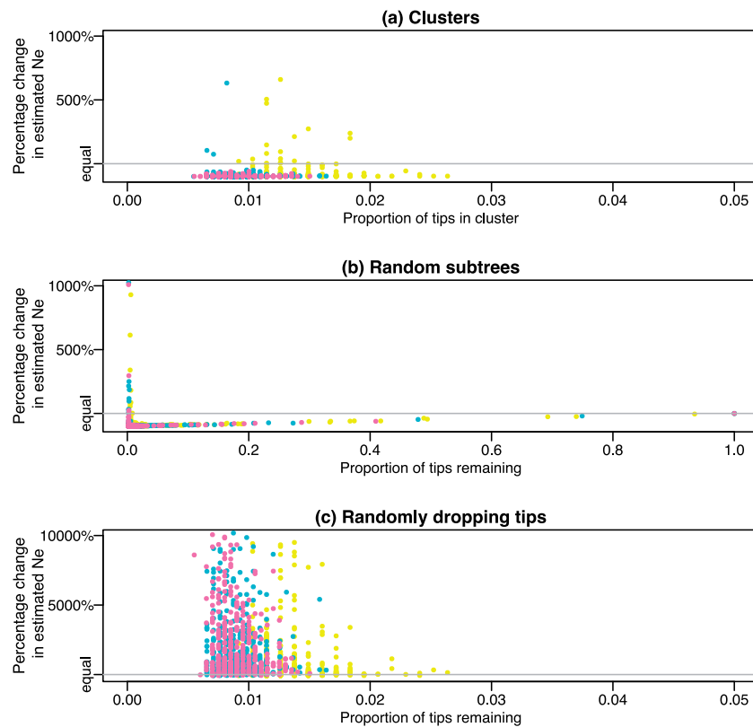
Figure 6. The effect on estimates of the present population size, N_e , in the HIV-like phylogenies when considering (a) clusters, (b) random subtrees and (c) tips dropped at random. Colours represent the PANGEA Village Simulation number: yellow = 0, green = 6, and pink = 7.
