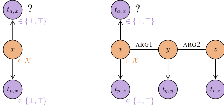
(a) Inferring if a is true of x , when there are no further pixies in the situation, and given the truth value for the predicate p . (b) Inferring if a is true of x , when x is part of a larger situation, and given the truth value for one predicate for each pixie in the situation.
