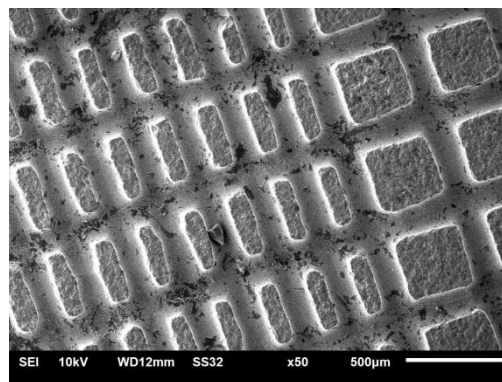
Fig. 1 – The image of the periodic structure on the surface of the wafer paratellurite (scanning electron microscope JEOL JSM-6610 LV)
