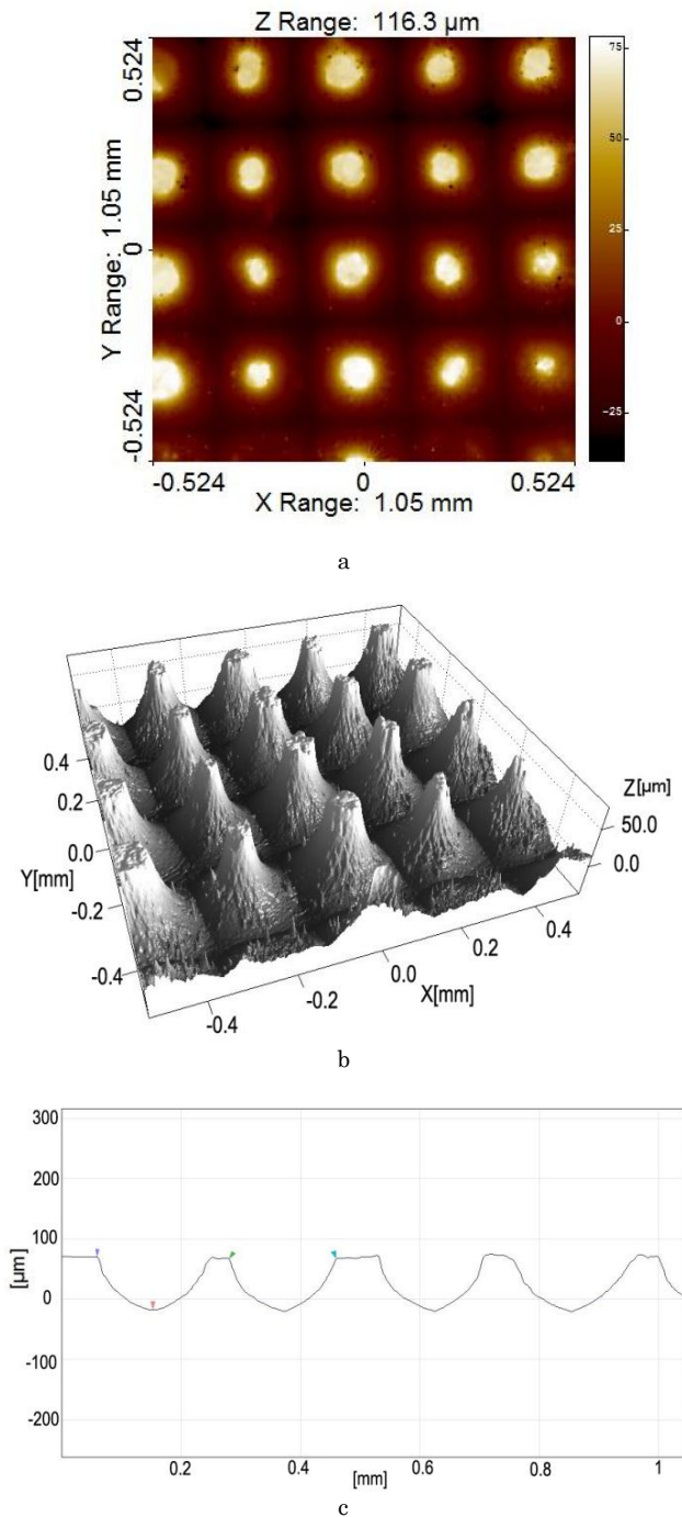
Fig. 2 – Image of the surface with a periodic structure 250 \times 250 micron formed by dissolving (a) its 3D profile (b) and 2D profile taken over the peaks centers (c)
