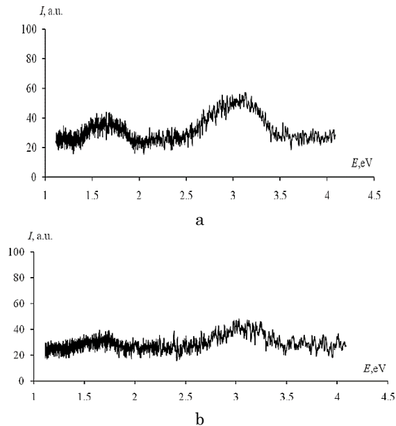
Fig. 2 – Photoluminescence spectra of ZrO_2 nanoparticles ablated at the Li intensity of 1010 \text{ W/m}^2 and annealed further during 3 hours at temperatures: a – 600 \text{ }^\circ\text{C} ; b – 1000 \text{ }^\circ\text{C}
