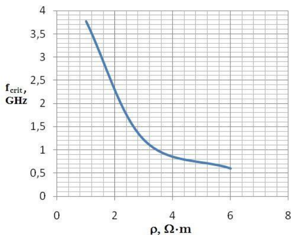
Fig. 3 – The dependence of the critical frequency of the electrical resistivity values typical for ferrites brands 700NM and 2000NM
