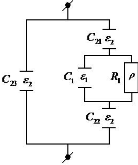
Fig. 1 – Model approximation of elemental composite shell as electric circuit
