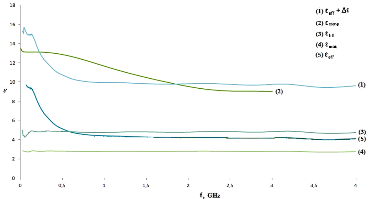
Fig. 2 – Dependence of permittivity on frequency for 1 – model proposed adding values according to the formula (6), 2 – composite sealant + 2000NM ferrite powder with a mass concentration 80 %, 3 – 2000NM ferrite powder, 4 – silicone sealant, 5 – model proposed
