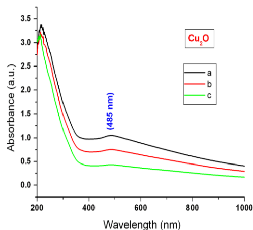
Fig. 5 – UV-VIS absorption spectra of Cu 2 O nanoparticles recorded (a) as synthesized (b) after one month (c) two months of Cu 2 O nanoparticles
