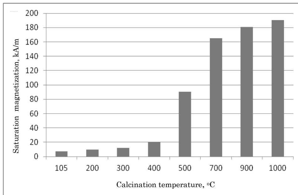
Fig. 4 – Dependence of the saturation magnetization of thermally treated galvanic sludge on the calcination temperature
