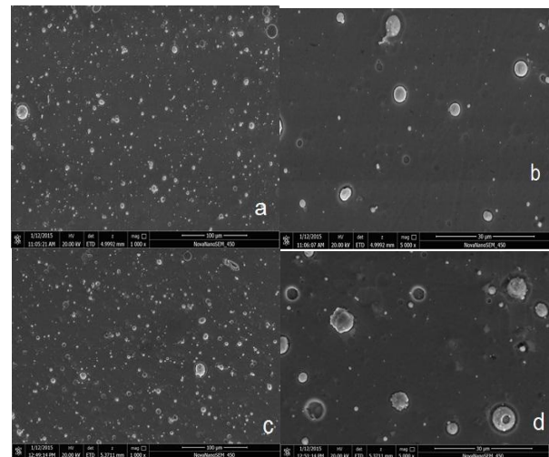
Fig. 3 – Surface view of the coatings from Series 2 ( \times 10^3 – a, \times 5 \cdot 10^3 – b) and Series 3 ( \times 10^3 – c, \times 5 \cdot 10^3 – d).
