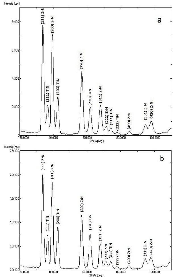
Fig. 2 – XRD spectra parts of the TiN/ZrN coatings from the Series 1 (a) and Series 2 (b).
