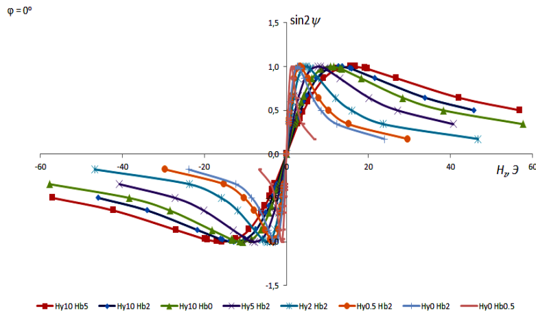
Fig. 4 – Graph of the function \sin 2\psi = f(H_z) for points on the surface of the MI conductor defined by \varphi = 0
