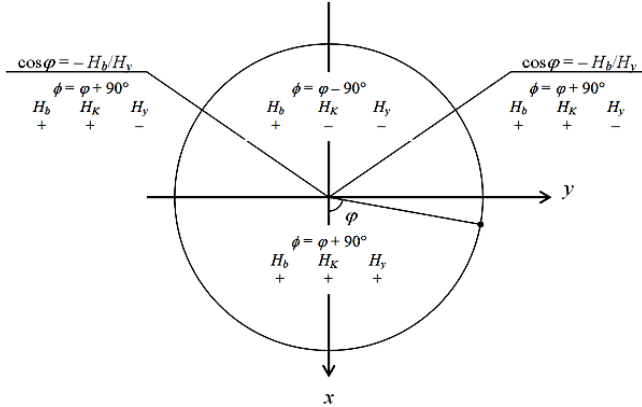
Fig. 2 – The solution domains to the angle \varphi
