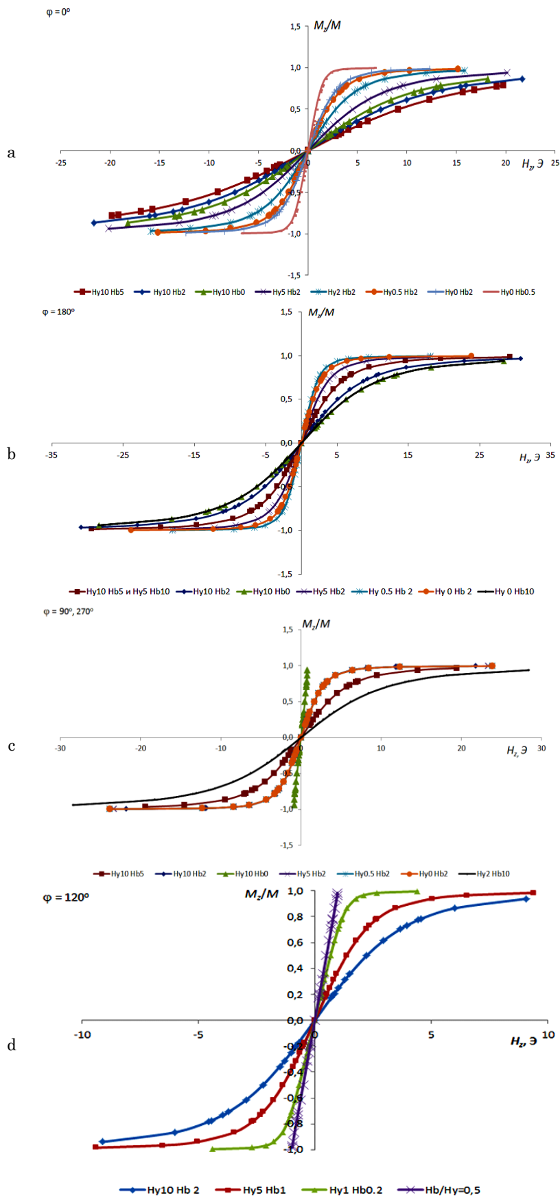
Fig. 3 – Relative value of the axial magnetization on the surface of wire with material parameters H_K = 1 Oe, 4\pi M = 500 G for different values of the external ( H_z and H_y ) and circular ( H_b ) magnetic fields (Oe). Characteristic points determined by following
