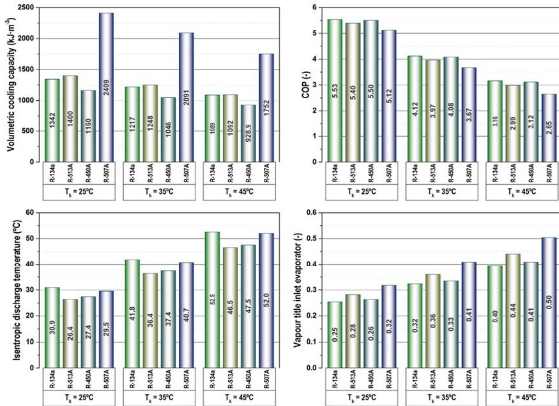
Figure 2. Thermodynamic VCC, COP, isentropic discharge temperature and vapour title at inlet of evaporator ( T_o = -14^\circ\text{C} )
