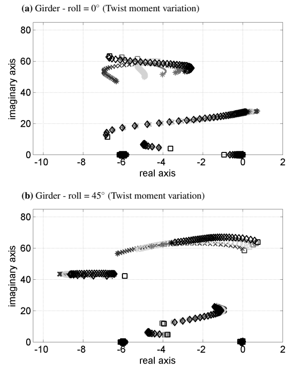
Fig. 23: Root loci for the Girder suspension system with constant normal trail ( cnt ) configuration. The twist moment coefficients are varied as 60%(blue ×), 80%(green o), 100%(magenta .), 120% (red +) and 140% (black ◇) of the nominal value. The speed is increased from 10 m/s (□) up to 80 m/s (*) at different roll angles.
