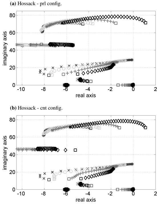
Fig. 22: Root loci of the Hossack suspension system with parallelogram ( prl ) and constant normal trail ( cnt ) configurations. The speed is increased from 10 m/s (□) up to 80 m/s (*) at different roll angles: 0° (blue ×), 15° (green o), 30° (red +) and 45° (black ◇).
