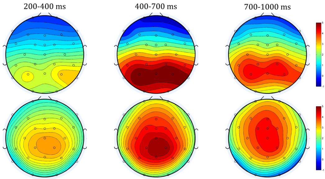
Figure 3. Topographic maps showing the mean amplitude (in \mu\text{V} ) enhancement for disgust (top) and fear (bottom) over neutral at each LPP time window (collapsed across condition).
