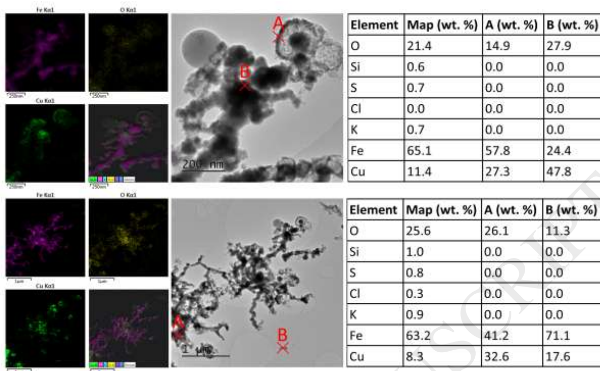
Figure 10. HRTEM-EDS maps along with spectra quantification data for the nZVI (and resultant Cu nanoparticles) following exposure to the pH buffered AMD for 4 hours. A nZVI concentration of 1.0 g/L was used. The pH buffer reagents comprised 0.1 g/L C_8H_5KO_4 and 0.005M HCl.
