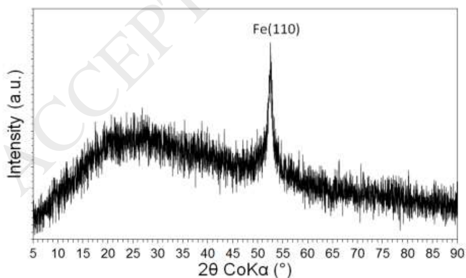
Figure 2. XRD spectra for the as-formed nZVI
