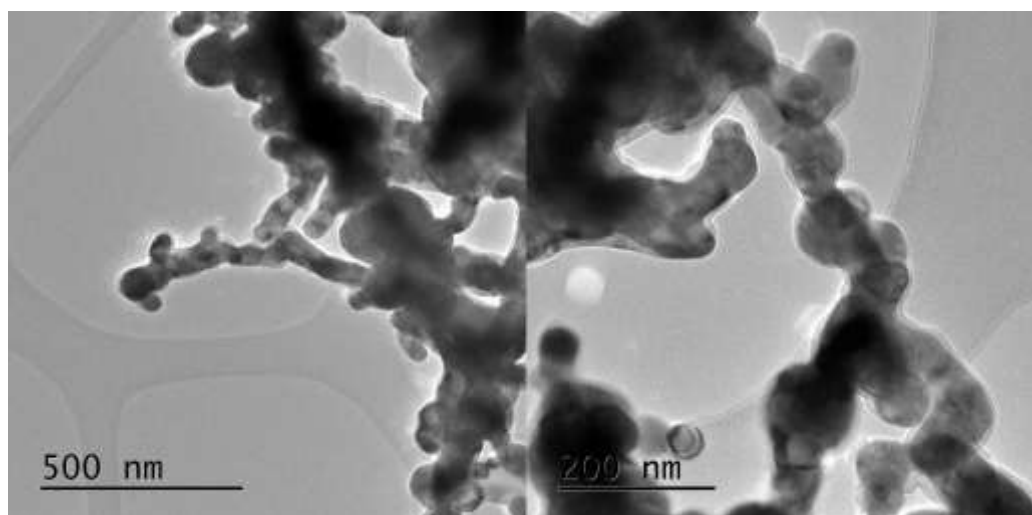
Figure 1. HRTEM images of the as-formed nZVI
