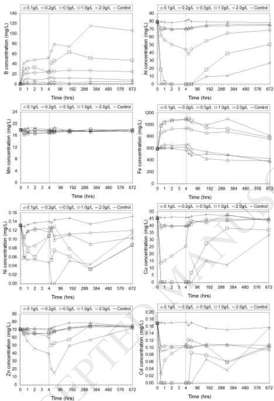
Figure 4. Aqueous concentrations of notable metal and metalloids as a function of time for the AMD when exposed to nZVI at 0.1, 0.2, 0.5, 1.0 and 2.0 g/L.
