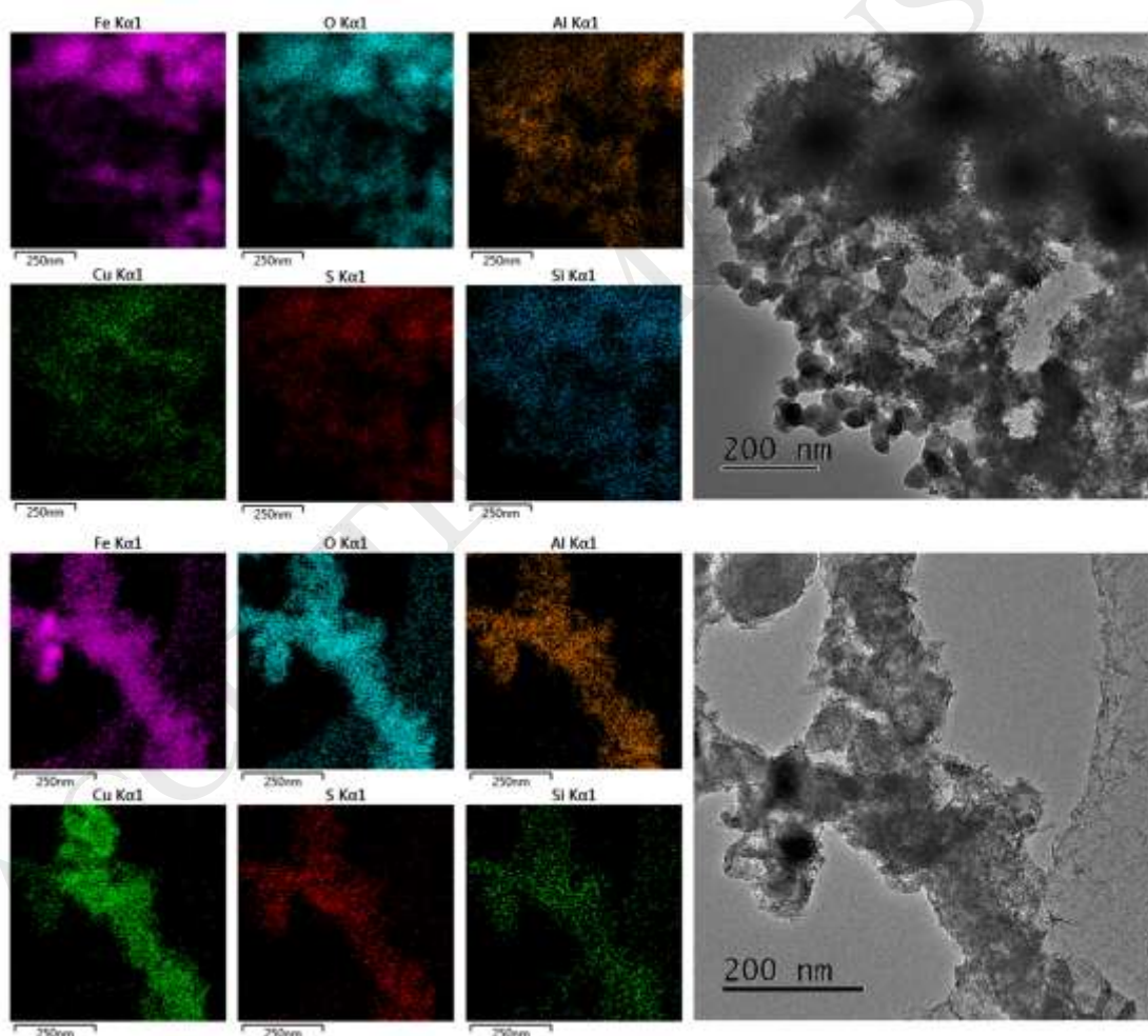
Figure 8. HRTEM and corresponding EDS maps of the six most abundant elements (by wt. %) of the nZVI after 4 hrs (top) and 24 hrs (bottom) exposure to the AMD (no pH buffer). Additional HRTEM images and EDS maps are displayed in Figures S6 and S7. A nZVI concentration of 1.0 g/L was used.
