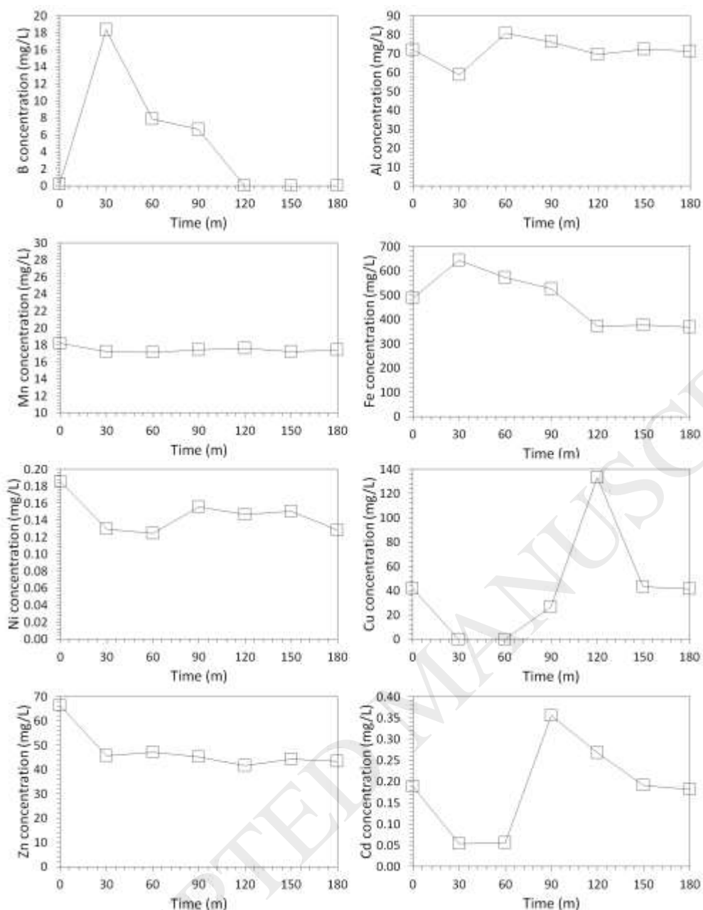
Figure 6. Changes in the aqueous concentration of notable metal and metalloids as a function of time for the AMD when fresh AMD has been used every 30 minutes. A nZVI concentration of 1.0 g/L was used.
