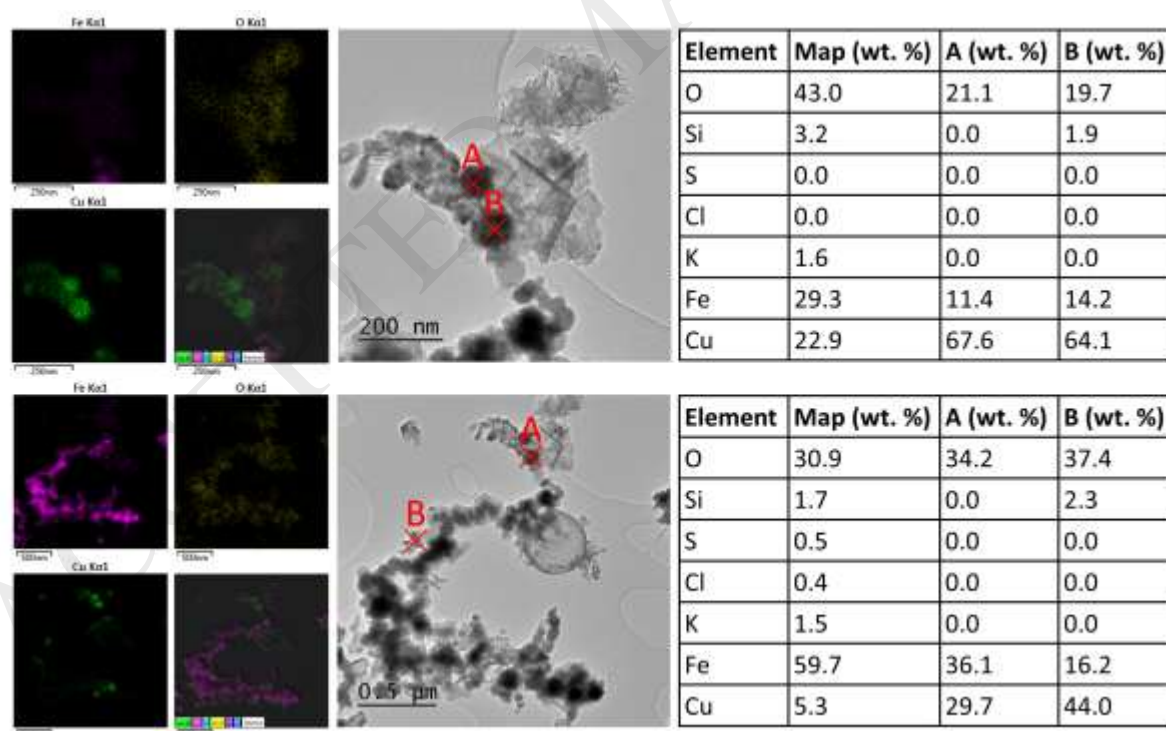
Figure 9. HRTEM-EDS maps along with spectra quantification data for the nZVI (and resultant Cu nanoparticles) following exposure to the pH buffered AMD for 1 hour. A nZVI concentration of 1.0 g/L was used. The pH buffer reagents comprised 0.1 g/L C_8H_5KO_4 and 0.005M HCl.
