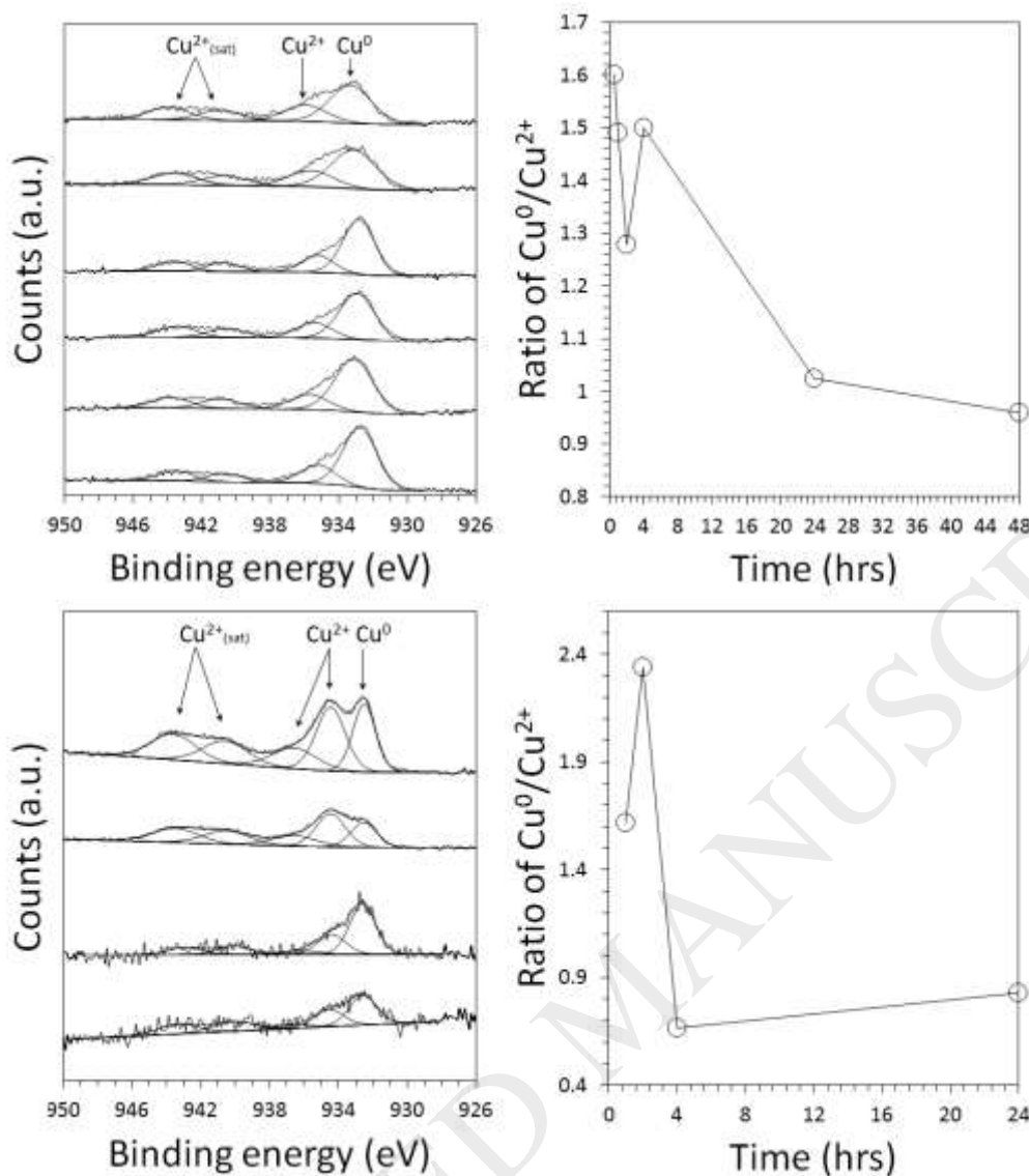
Figure 7. Curve fitted XPS Cu 2p_{3/2} spectra for nZVI extracted from the unbuffered (top) and pH buffered* (bottom) AMD after 0.5, 1, 2, 4, 24 and 48 hrs and 1, 2, 4 and 24 hrs (stacked from bottom to top) respectively along with corresponding ratios of \text{Cu}^0/\text{Cu}^{2+} calculated by integrating the area under each corresponding curve fitted photoelectron peak. A nZVI concentration of 1.0 g/L was used. *The pH buffer reagents comprised 0.1 g/L \text{C}_8\text{H}_5\text{KO}_4 and 0.005M HCl.
