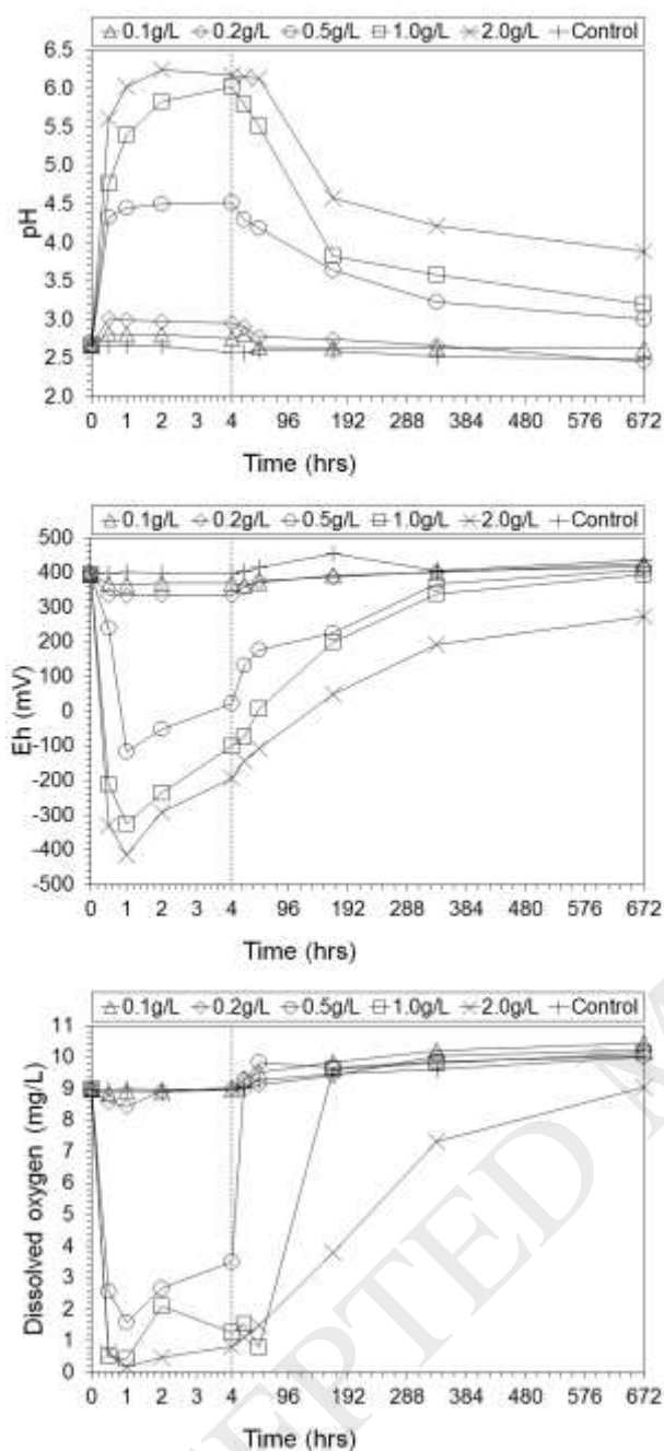
Figure 3. Changes in pH, Eh and DO as a function of time for the unbuffered batch systems.
