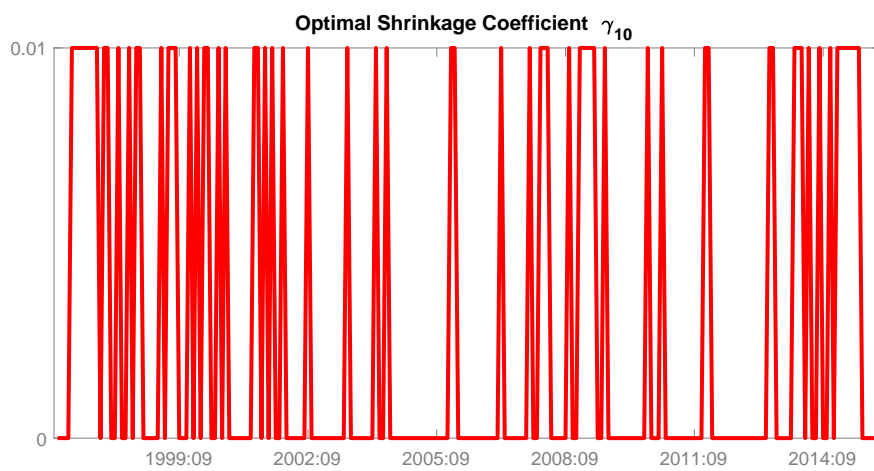
Figure 12: Values of the shrinkage factor of VIX.
