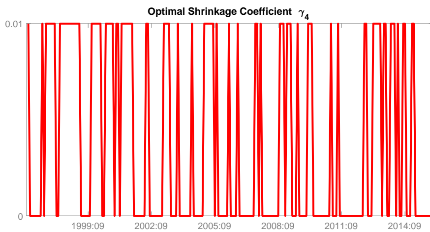
Figure 6: Values of the shrinkage coefficient for EXPECTATIONS.
