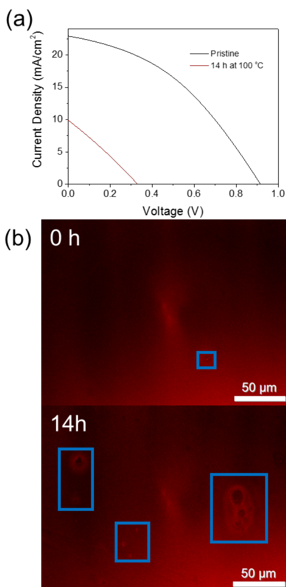
Figure 8. (a) I-V curves of a \text{CH}_3\text{NH}_3\text{PbI}_3 PSC before (black) and after (red) heating at 100\text{ }^{\circ}\text{C} for 14 h. (b) Fluorescence microscopy images of the \text{CH}_3\text{NH}_3\text{PbI}_3 PSC before and after heating at 100\text{ }^{\circ}\text{C} for 14 h. The blue box highlight the visible pinhole defects.
