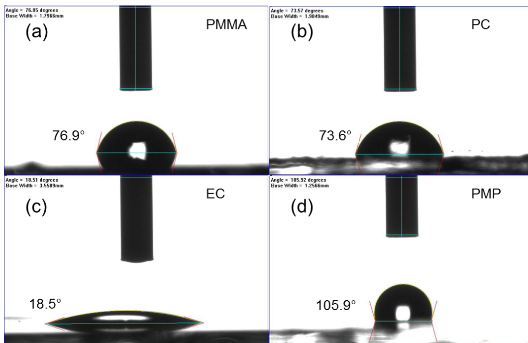
Figure 5. Determination of the surface hydrophobicity of polymer films coated on glass slides using contact angle measurements: (a) PMMA, (b) PC, (c) EC and (d) PMP.
