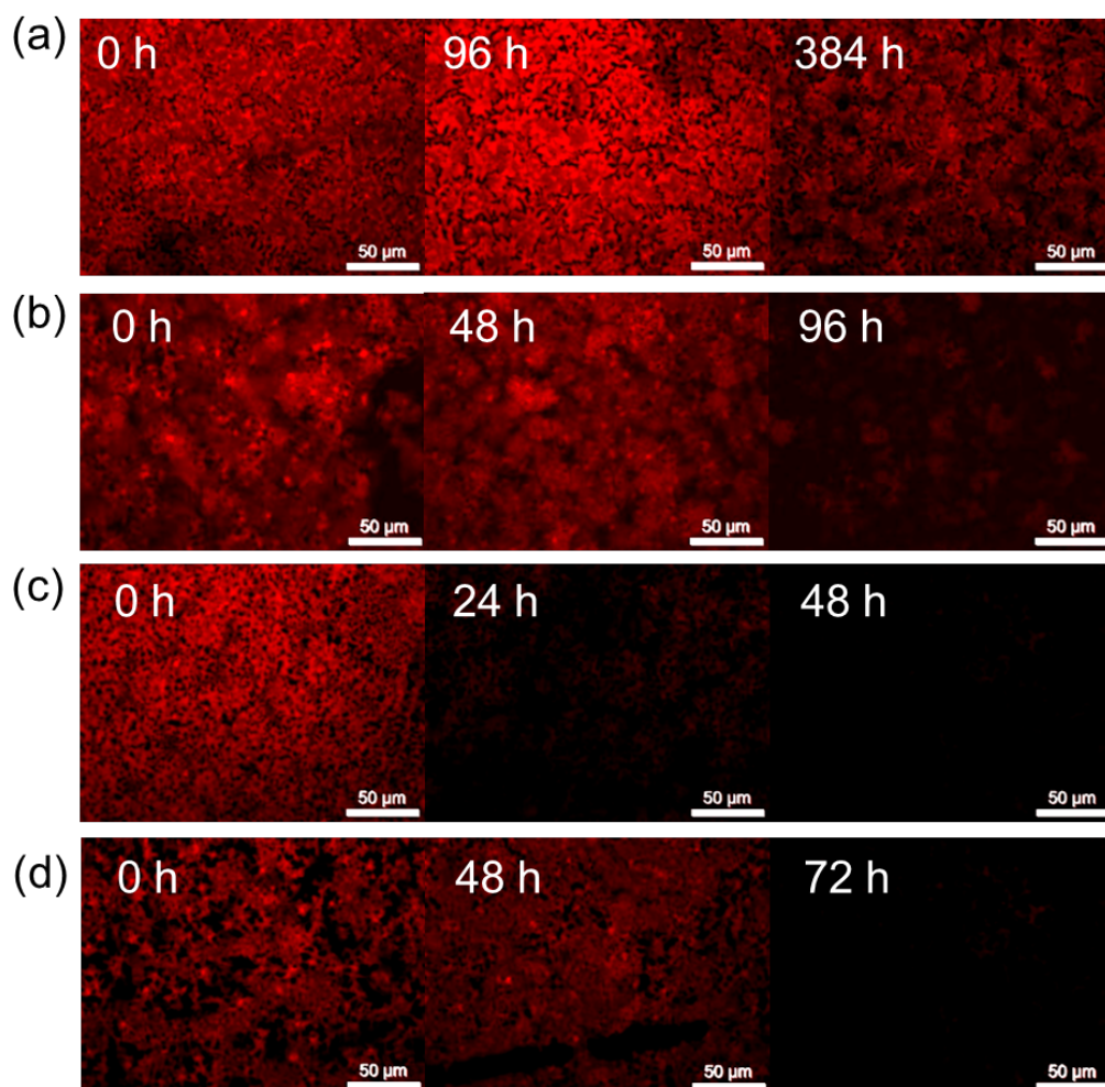
Figure 6. Thermal degradation of polymer encapsulated \text{CH}_3\text{NH}_3\text{PbI}_{3-x}\text{Cl}_x films at 60 °C as a function of time monitored by fluorescence microscopy. \text{CH}_3\text{NH}_3\text{PbI}_{3-x}\text{Cl}_x degradation is accompanied by a decrease in emission intensity and hence darkening of the image. (a) PMMA shows negligible degradation after 384 h, (b) PC degrades completely after 96 h, (c) EC shows an onset of degradation after 24 h and (d) PMP shows complete degradation after 72 h.
