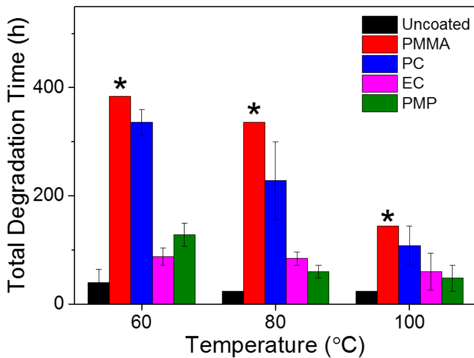
Figure 4. The mean times required for complete degradation of the UV/Vis absorption band edge (750 nm) for pristine and polymer-encapsulated \text{CH}_3\text{NH}_3\text{PbI}_{3-x}\text{Cl}_x films as a function of degradation temperature. The error bars represent the standard deviation of three measurements. The * indicates that at that time of characterisation there was still no indication of degradation.
