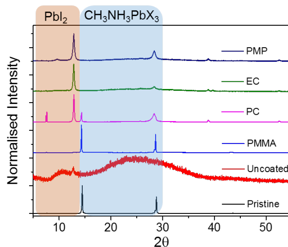
Figure 2. PXRD patterns of uncoated and polymer-encapsulated \text{CH}_3\text{NH}_3\text{PbI}_{3-x}\text{Cl}_x films following thermal degradation in 60^\circ\text{C} in air for 432 h. The PXRD pattern of the pristine uncoated \text{CH}_3\text{NH}_3\text{PbI}_{3-x}\text{Cl}_x film prior to thermal degradation is also shown for comparison (black line). After 432 h, the uncoated film displayed total degradation, such that the observed pattern predominantly represents that of the amorphous glass substrate.
