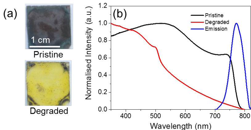
Figure 1. Comparison of the optical properties of a pristine and thermally degraded (60 °C for 72 h in air) \text{CH}_3\text{NH}_3\text{PbI}_{3-x}\text{Cl}_x film (~500 nm thick). (a) Photograph illustrating the colour change that occurs upon degradation. (b) Normalised UV/Vis absorption spectrum of an uncoated \text{CH}_3\text{NH}_3\text{PbI}_{3-x}\text{Cl}_x film before (black line) and after (red line) thermal degradation. The photoluminescence spectrum (blue line) of the pristine film of \text{CH}_3\text{NH}_3\text{PbI}_{3-x}\text{Cl}_x ( \lambda_{\text{ex}} = 500 nm) is also shown.
