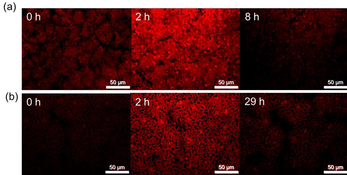
Figure 7. Thermal degradation of pristine and EC-encapsulated \text{CH}_3\text{NH}_3\text{PbI}_{3-x}\text{Cl}_x films at 60 °C as a function of time, as monitored by epifluorescence microscopy. (a) The uncoated \text{CH}_3\text{NH}_3\text{PbI}_{3-x}\text{Cl}_x film exhibits significant darkening after 8 h. (b) The EC-encapsulated film exhibits significant darkening after 29 h. After 2 h at 60 °C, the fluorescence of both films is more intense due to the removal of solvent and additional annealing.
