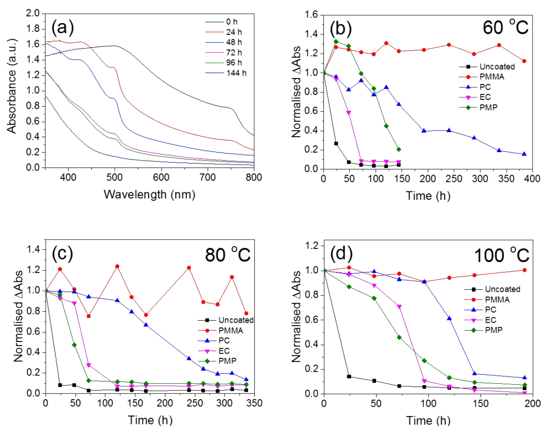
Figure 3. Thermal degradation of pristine and polymer-encapsulated \text{CH}_3\text{NH}_3\text{PbI}_{3-x}\text{Cl}_x films followed by ex-situ UV/Vis absorption spectroscopy. (a) UV/Vis absorption spectra of PMP-coated films degraded at 80 °C as a function of time, t . (b) Difference in absorbance between 750 nm and 800 nm ( \Delta Abs) as a function of time, normalised to t = 0 h for films degraded at 60 °C in air, (c) 80 °C in air and (d) at 100 °C in air. The solid lines serve only to guide the eye.
