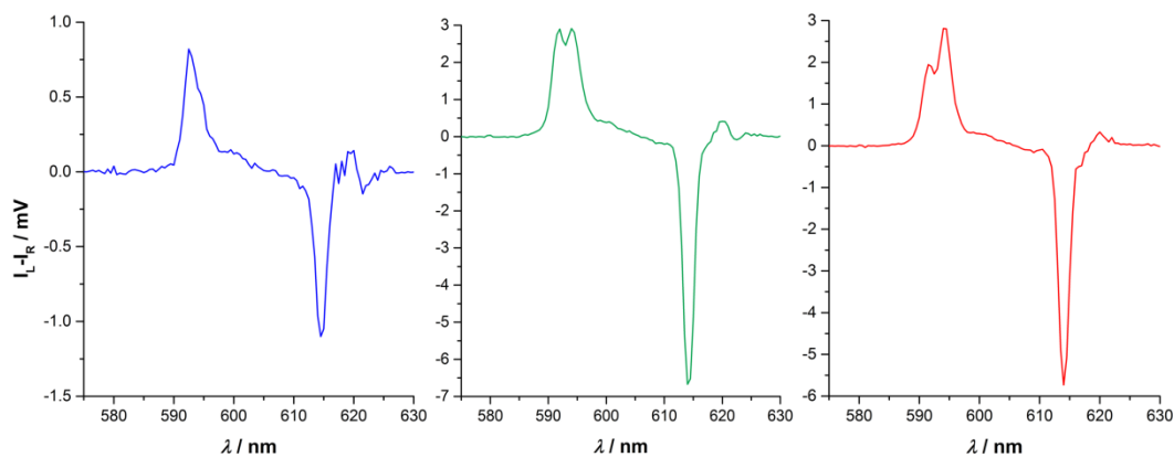
Figure 3.35 Circularly polarised luminescence spectra of the \Delta J = 1 and 2 region for \Delta -[EuL 7 ] in H 2 O ( blue ), MeOH ( green ) and DMSO ( red ) ( \lambda_{\text{exc}} = 272 nm, 295 K). The maximum g_{\text{em}} values in the \Delta J = 1 manifold are +0.07 in water, and +0.18 in DMSO and MeOH.
