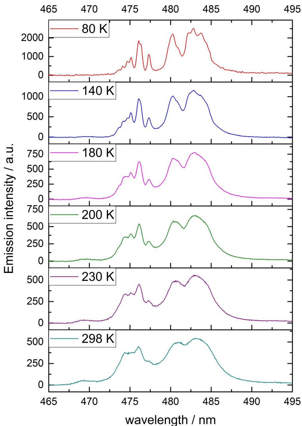
Figure 3.30 Variable temperature emission spectra of [DyL 7 ] in the ^4F_{9/2} \rightarrow ^6H_{15/2} manifold showing increased resolution as temperature is decreased (1:4 v/v methanol:ethanol, \lambda_{\text{exc}} 272 nm).
