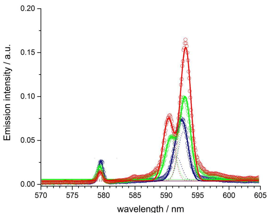
Figure 3.34 Expanded emission spectra of [EuL 7 ] in the \Delta I = 0 and 1 regions in water ( blue ), methanol ( green ) and DMSO ( red ) (295 K, \lambda_{\text{exc}} 272 nm); raw data is shown as open circles, fitted spectra as solid lines and deconvoluted Gaussians as dotted lines.
