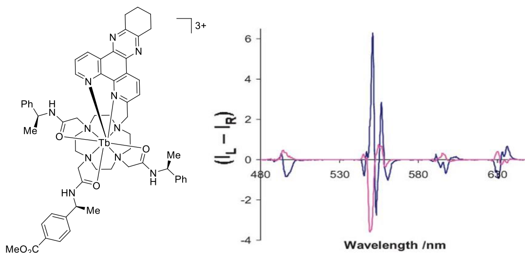
Figure 1.33 The ( SSS )- \Delta enantiomer ( left ) and its CPL spectrum in the absence ( blue ) and presence ( pink ) of 2 equivalents of bovine serum albumin (295 K, D 2 O, \lambda_{\text{exc}} 348 nm). Reproduced from Ref. [87] with permission from The Royal Society of Chemistry.
