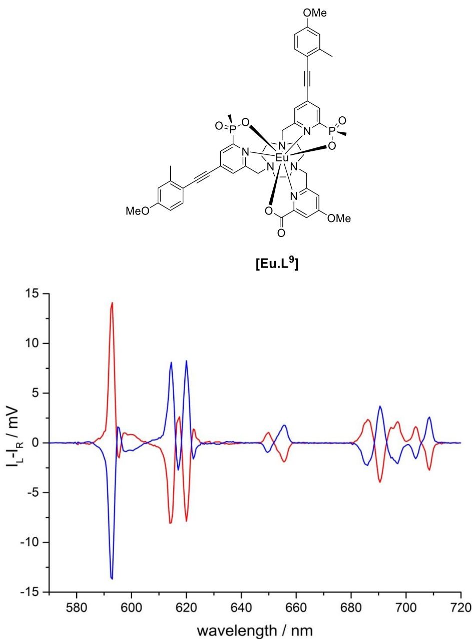
Figure 2.23 The CPL spectra of the \Delta -(red) and \Lambda -(blue) enantiomers of [EuL 9 ] (MeOH, 295 K, \lambda_{\text{exc}} 340 nm).
