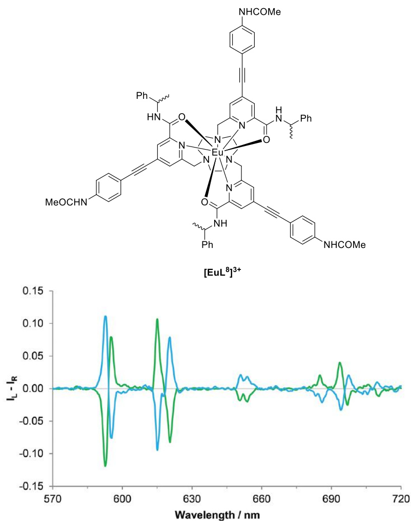
Figure 2.22 The CPL spectra of the S-\Delta (green) and R-\Lambda (blue) enantiomers of [\text{EuL}^8]^{3+} ( \text{H}_2\text{O} , 295 K, \lambda_{\text{exc}} 348 nm). Reproduced from Ref. [75] with permission from The Royal Society of Chemistry.
