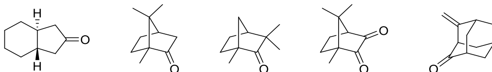
Figure 1.17 A selection of CPL-active chiral ketones; from left to right: (+)-( S,S )- trans - \beta -hydrindanone, ( 1R )-camphor, ( 1R )-fenchone, ( 1R )-camphorquinone and ( 1S , 3R )-4-methyleneadamantan-2-one.
