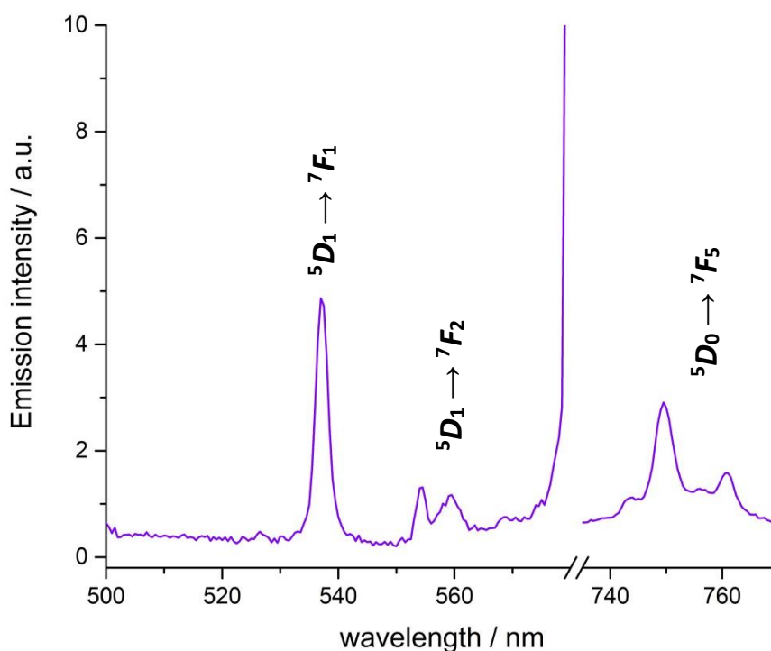
Figure 2.20 Expanded total emission spectrum for [EuL 2 ] showing some transitions rarely observed in solution for molecular systems (MeOH, 295 K, 5 \mu M complex, \lambda_{exc} 343 nm, 5 scans averaged).
