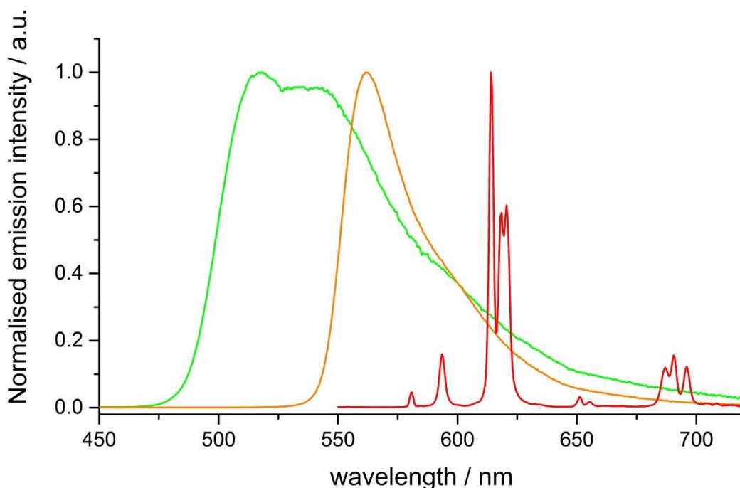
Figure 2.37 Normalised emission spectra of fluorescein ( green , MeOH, \lambda_{\text{exc}} 354 nm, 295 K), rhodamine 6G ( orange , MeOH, \lambda_{\text{exc}} 348 nm, 295 K) and [EuL 1 ] ( red , MeOH, \lambda_{\text{exc}} 356 nm, 295 K).
