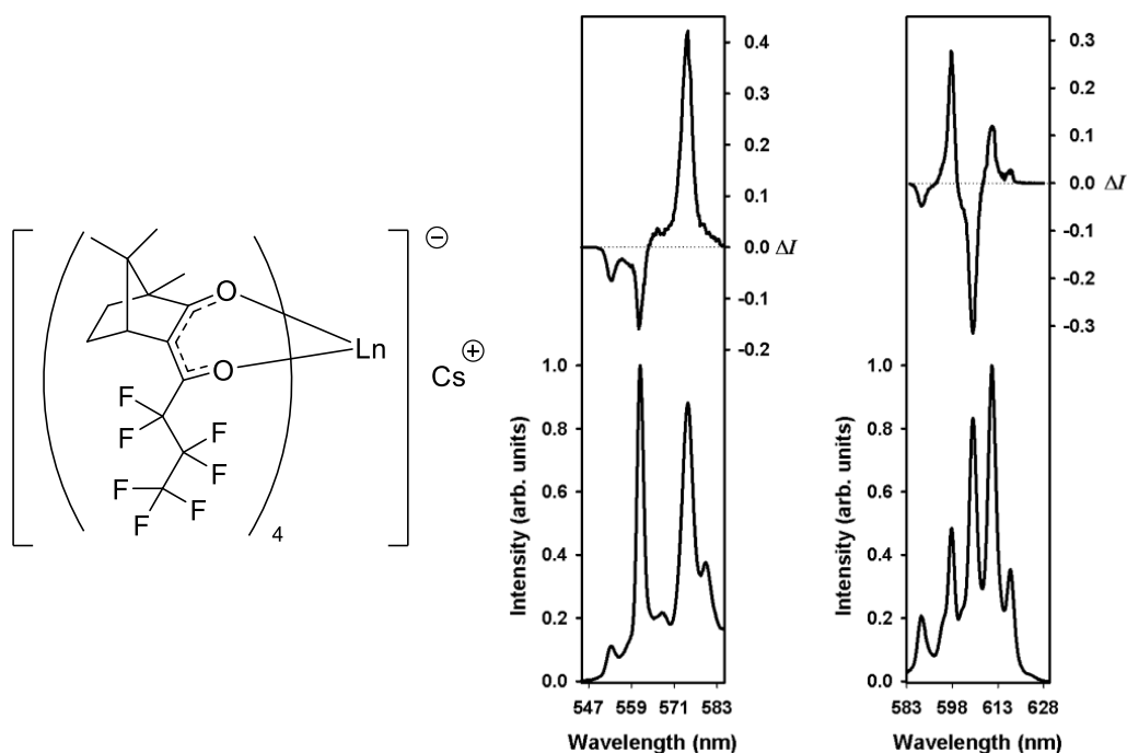
Figure 1.28 The structure of Cs[Ln((+)-hfbcb) 4 ] (left) and the CPL spectra of Cs[Sm((+)-hfbcb) 4 ] in the ^4G_{4/2} \rightarrow ^6H_{5/2} and ^4G_{4/2} \rightarrow ^6H_{7/2} transitions (right, CHCl 3 , 295 K, \lambda_{\text{exc}} 338 nm) Reprinted with permission from Ref. [70]. Copyright (2011) American Chemical Society.
