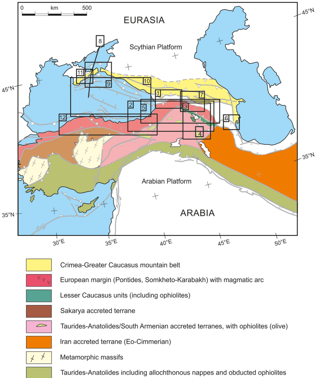
Fig. 1. Tectonic map of the Black Sea–Caucasus domain and surrounding areas, modified from Sosson et al. (2015), showing the field locations of studies reported in this Special Publication: 1, Adamia et al. (2015); 2, Hässig et al. (2015); 3, Danelian et al. (2015), Sahakyan et al. (2016) and Cavazza et al. (2015); 4, Avagyan et al. (2016); 5, Meijers et al. (2015); 6, van der Boon et al. (2015); 7, Alania et al. (2015); 8, Starostenko et al. (2016); Sydorenko et al. (2016); 9, Gobarenko et al. (2015); 10, Nikishin et al. (2015 b ); 11, Sheremet et al. (2016 b ); and 12, Hippolyte et al. (2015).
