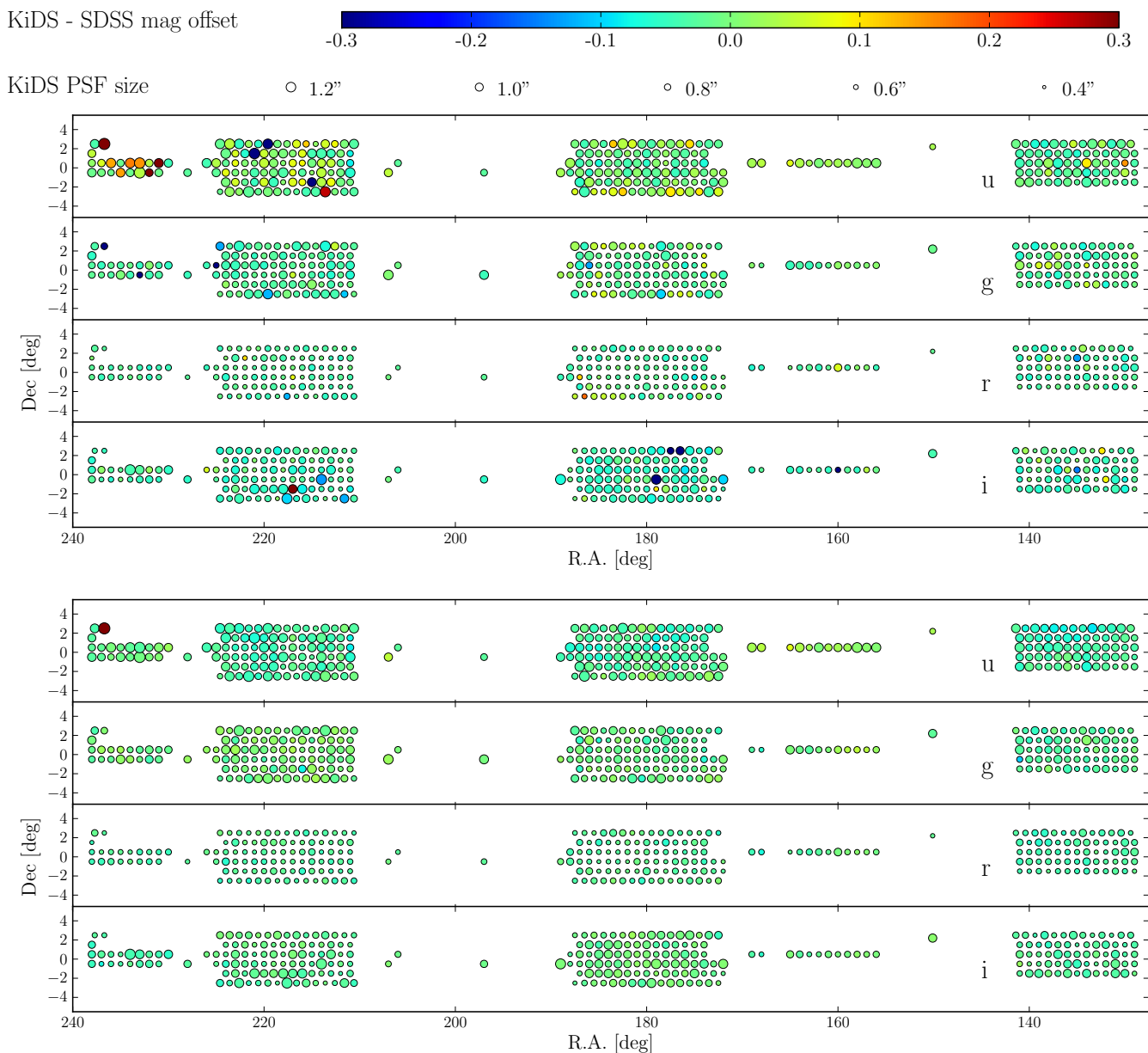
Fig. 4. Comparison of KiDS GAAP photometry before and after homogenization to SDSS DR13 for all tiles in KiDS-North as function of right ascension and declination. Top : the magnitude offsets with respect to SDSS before applying photometric homogenization are indicated by the color scaling. The size of the circles represent the average PSF size in each coadded image. From top to bottom the panels correspond to the u , g , r , and i filters. Bottom : same as top panel, but after applying photometric homogenization.
