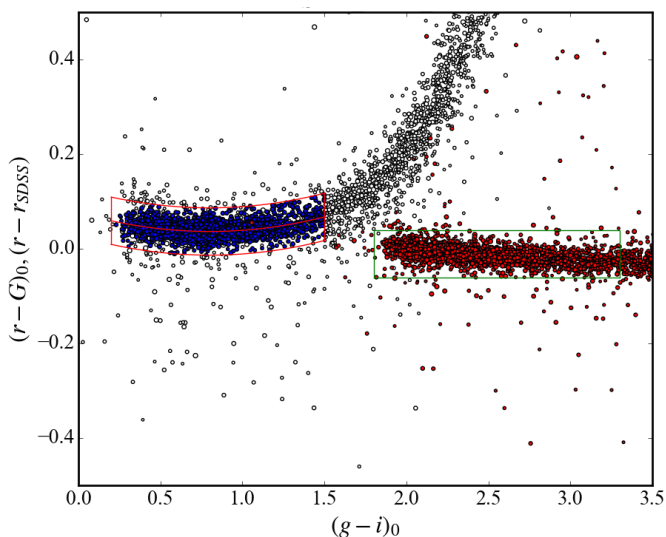
Fig. 6. Comparison of KiDS r -band GAaP photometry to Gaia DR1 G -band and SDSS DR9 r -band photometry. Stars with dereddened g-i colours, based on colour-calibrated KiDS GAaP data ( x -axis), between 0.2 and 1.5 are selected to iteratively derive the median photometric offsets (r-G)_0 (left sequence) and (r-r_{\text{SDSS}}) (right sequence). The latter sequence of data points is shifted by 1.6 mag in (g-i)_0 for clarity. The red and green outlines show the regions encompassing the data points used in the final iteration of each fit.
