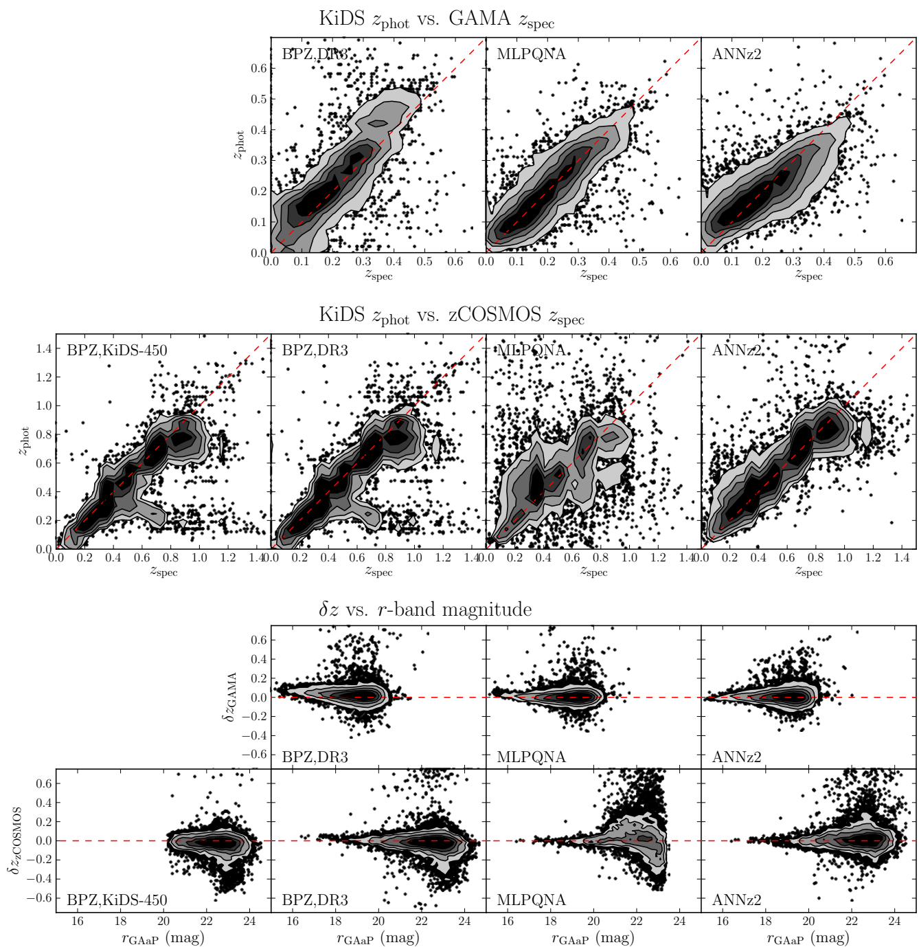
Fig. 11. Comparison of photometric redshifts to spectroscopic redshifts. Top: direct comparisons of best-guess photo- z 's against GAMA DR2 spec- z 's. From left to right the panels show the BPZ photo- z 's in the DR3 multi-band catalogue, the MLPQNA photo- z 's and the ANNz2 photo- z 's. The red dashed line corresponds to z_B = z_{\text{spec}} and the contours are chosen randomly to enhance the clarity of the figures. Centre: same as the top row, but now comparing to zCOSMOS bright DR3 spec- z 's and with on the left a panel added for the BPZ photo- z 's included in the KiDS-450 shear catalogue. Bottom: normalized photo- z error \delta z versus r -band magnitude. The panels in the first row show the comparison to GAMA DR2 and the second row the comparison to zCOSMOS bright DR3. The order of the panels follows the order in the top and centre rows.
