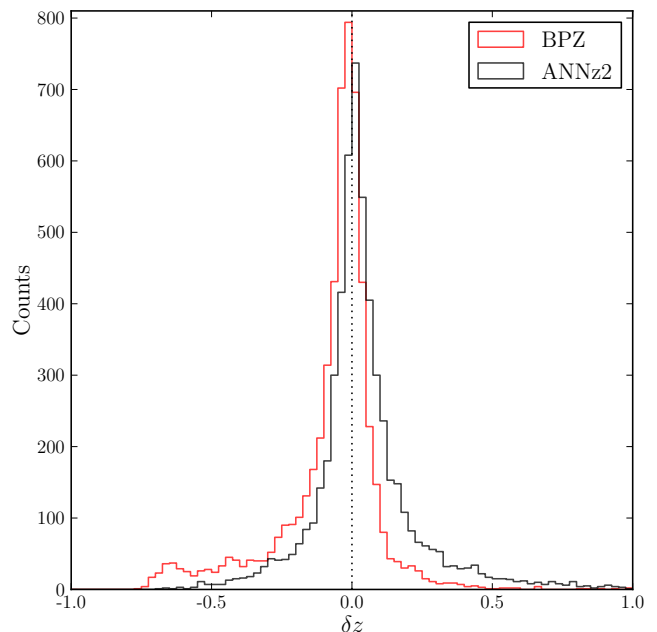
Fig. 10. Comparison of normalised photometric redshift errors for ANNz2 (black) and BPZ (red) in the CDFS field.
