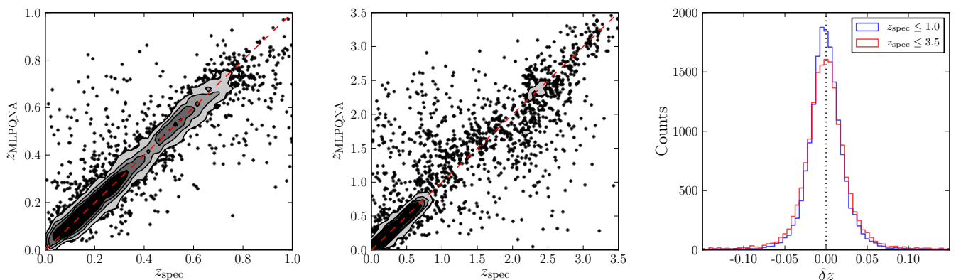
Fig. 9. Results of the MLPQNA photo- z experiments. Left: Scatter plot of z_{\text{spec}} vs z_{\text{phot}} for the experiment limiting z_{\text{spec}} between 0.01 and 1. Centre: Same as the left panel but for z_{\text{spec}} between 0.01 and 3.5. Right: Histograms of the residual distribution for the experiment with 0.01 < z_{\text{spec}} < 1.0 (blue) and 0.01 < z_{\text{spec}} < 3.5 (red).
