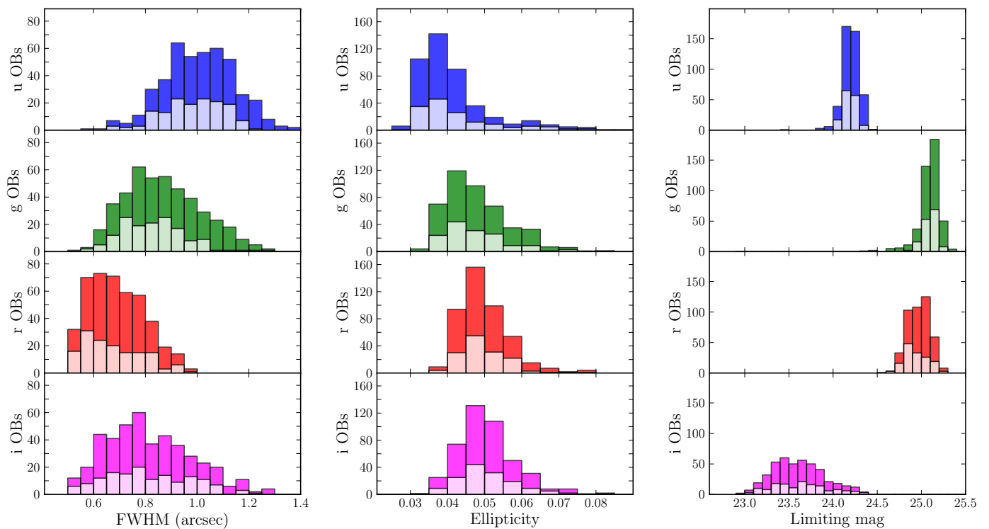
Fig. 2. Data quality for KiDS-ESO-DR1 -DR2 and -DR3. Left: average PSF size (FWHM) distributions; center: average PSF ellipticity distributions; right: limiting magnitude distributions ( 5\sigma AB in 2'' aperture). The distributions are per filter: from top to bottom u , g , r , and i , respectively. The full histograms correspond to the 440 tiles included in the DR3 multi-band catalog, while the lighter portions of the histograms correspond to fraction (148 tiles) previously released in KiDS-ESO-DR1 and -DR2.
