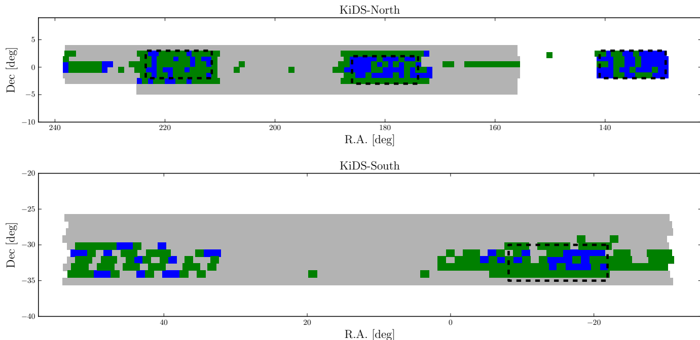
Fig. 1. Sky distribution of survey tiles released in KiDS-ESO-DR3 (green) and in the previous releases KiDS-ESO-DR1 and -DR2 (blue). The multi-band source catalogue covers the combined area (blue + green) and the full KiDS area is shown in grey. Top: KiDS-North. Bottom: KiDS-South. Black dashed lines delineate the locations of the GAMA fields; the single pointing at RA=150° is centered at the COSMOS/CFHTLS D2 field.
