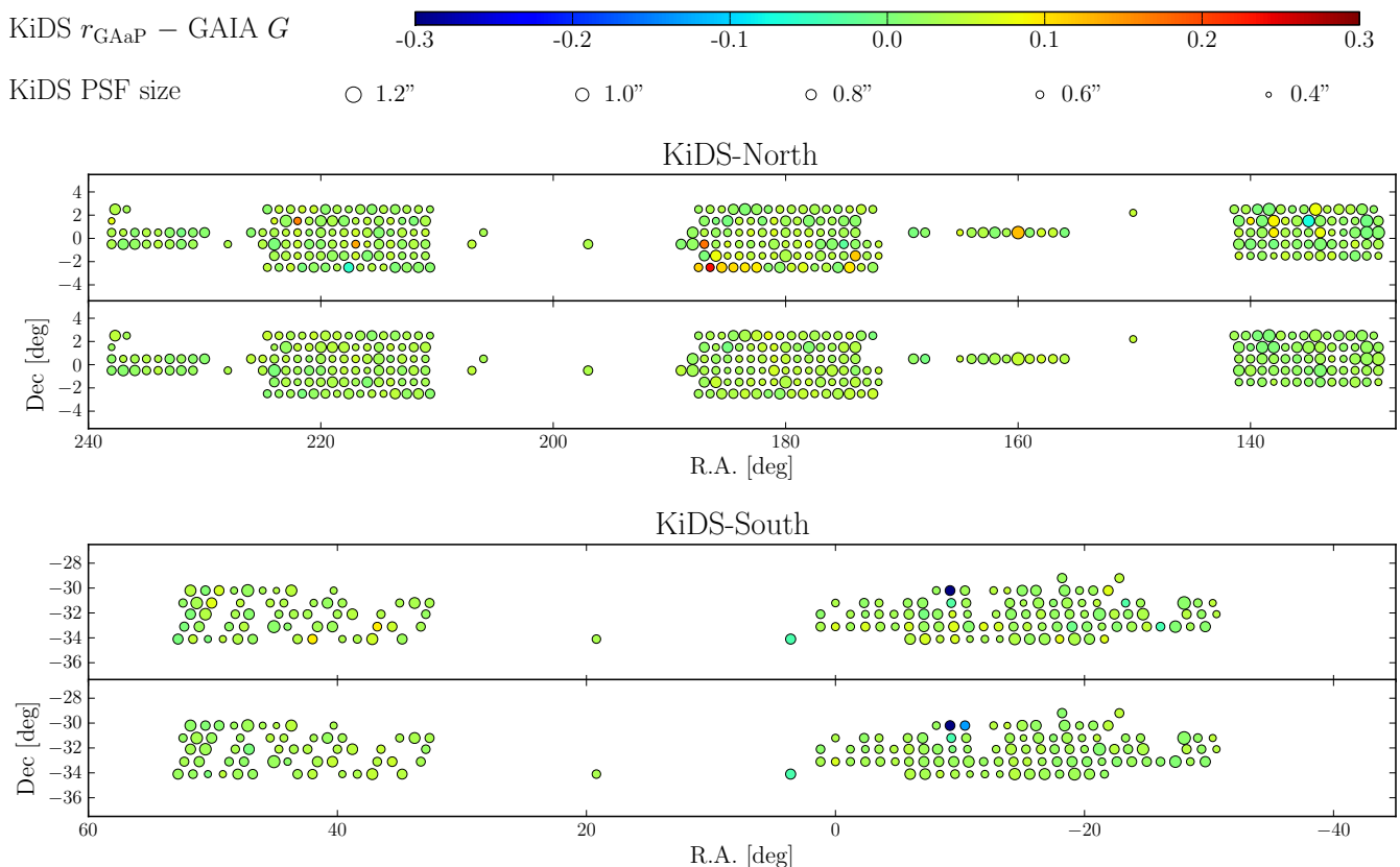
Fig. 7. Comparison of KiDS r -band to Gaia G -band photometry as function of position on the sky. The per-tile median photometric offset ( r_{\text{GaAP}} - G ) is indicated by the color scale, while the marker size corresponds to the mean seeing in the KiDS r -band image. Top: Comparison for KiDS-North, with in the top and bottom subpanels showing the offsets before and after applying the photometric homogenization, respectively. Bottom: same as the top panel, but now for KiDS-South.
