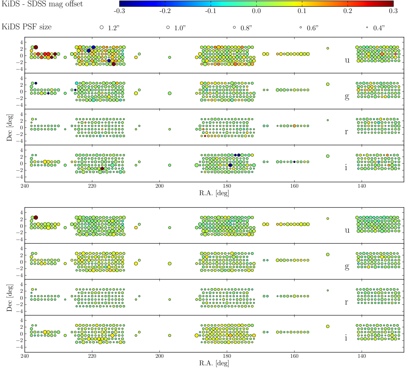
Fig. 5. Comparison of KiDS 10'' aperture-corrected photometry before and after homogenization to SDSS DR13 for all tiles in KiDS-North as function of right ascension and declination. Top : the magnitude offsets with respect to SDSS before applying photometric homogenization are indicated by the color scaling. The size of the circles represent the average PSF size in each coadded image. From top to bottom the panels correspond to the u , g , r , and i filters. Bottom : same as top panel, but after applying photometric homogenization.
