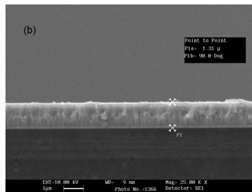
Fig. 4 – (a) a typical EDX spectrum obtained from SnO 2 :Sb thin films on silicon wafers by EDX analysis and (b) SEM cross section view of Sb :SnO 2 thin film deposited by co evaporation of Sb and Sn
